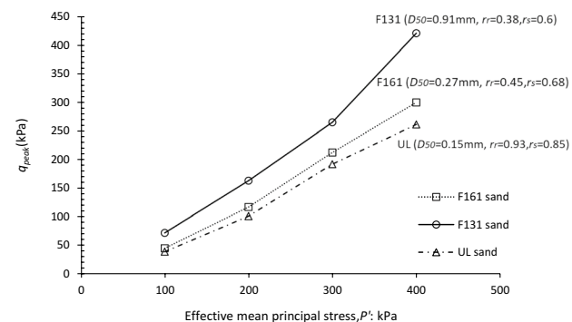
Fig. 8 The peak strength of sands
