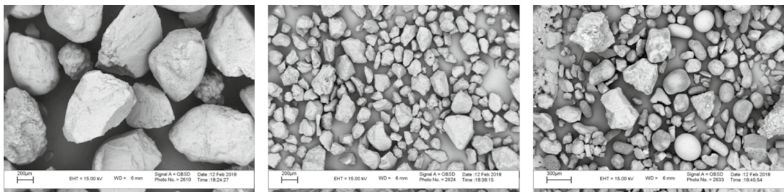
Fig. 2 Particle size distribution, shape and texture of test specimen constituents a F131, b 161 and c UL
