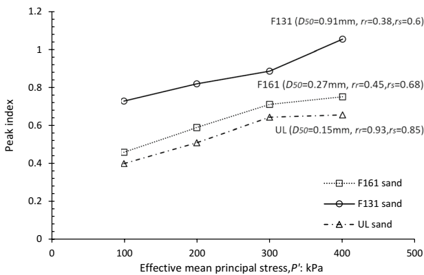
Fig. 11 Demonstrates the variation of the peak strength index
