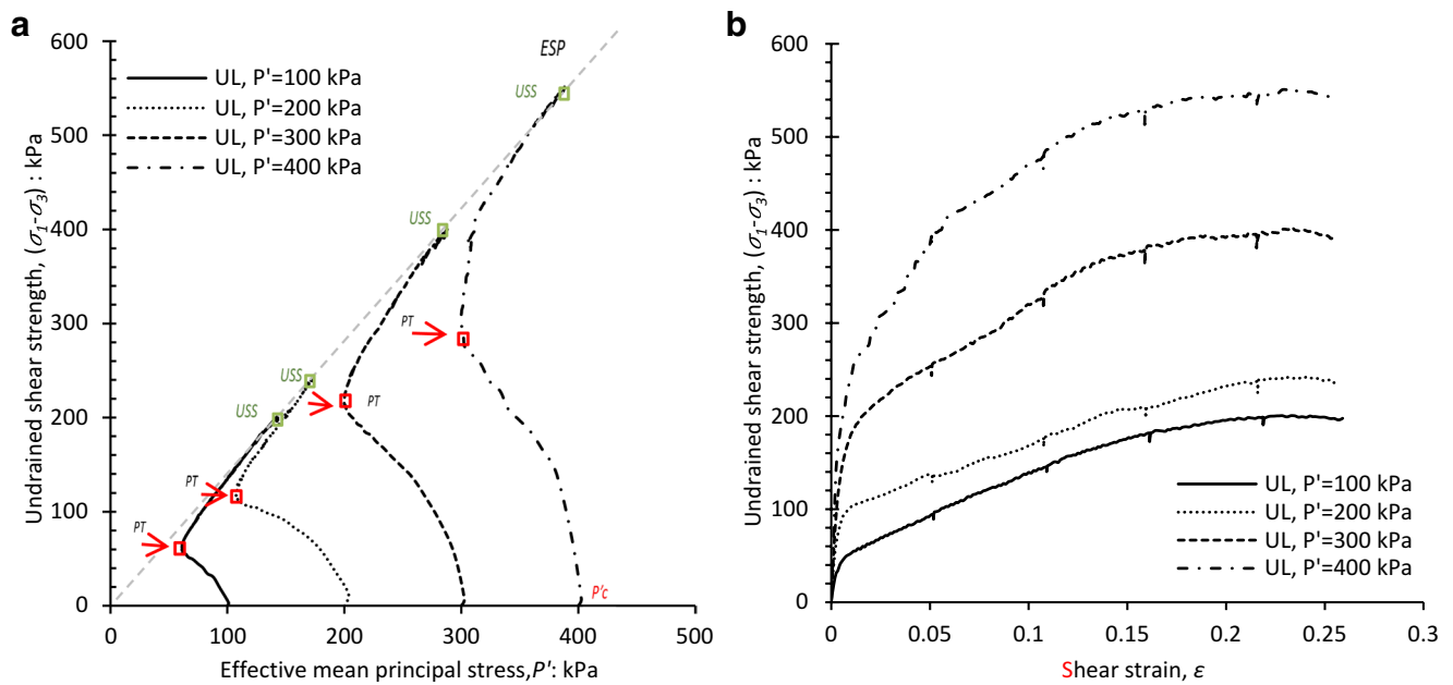
Fig. 5 Undrained behaviour of UL sand a stress path on q - p' space; b stress-strain behaviour
