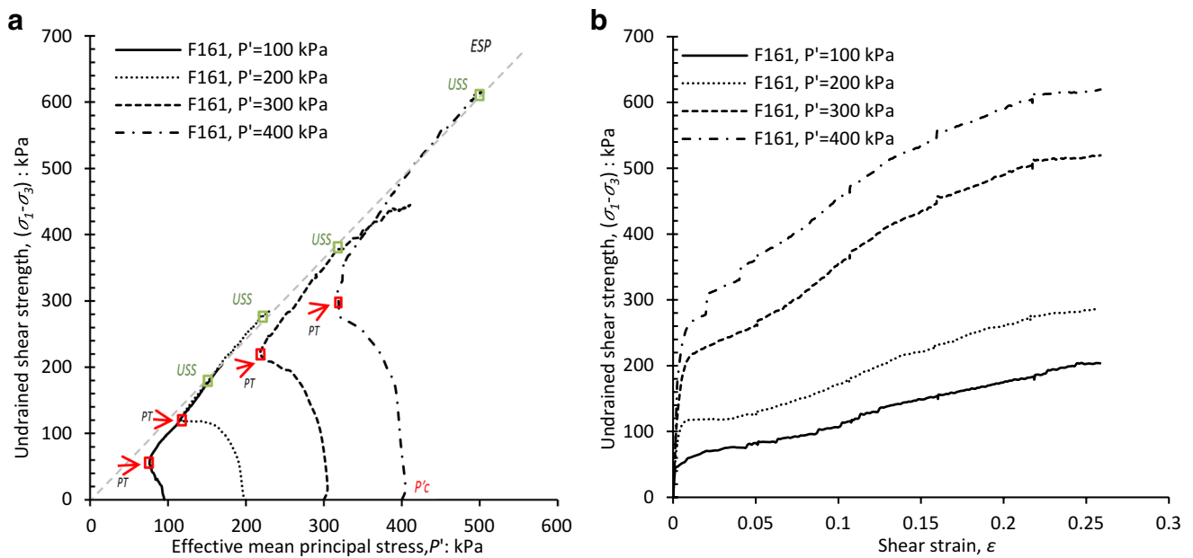
Fig. 3 Undrained behaviour of F161 sand a stress path on q-p' space; b stress–strain behaviour
