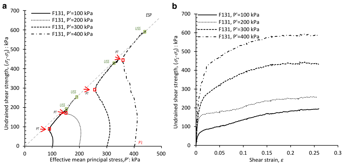
Fig. 4 Undrained behaviour of F131 sand a stress path on q-p' space; b stress–strain behaviour
