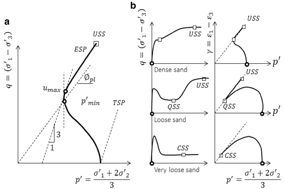
Fig. 1 a Phase transformation state during undrained shearing of sand; b steady states during undrained shearing of sand (after editorial adjustments [30])
