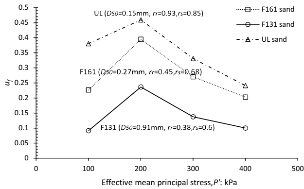
Fig. 10 Demonstrates the variation of the flow potential index
