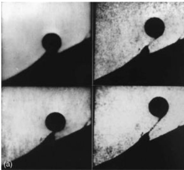
Fig. 5 Selected frames from a high-speed photographic sequence showing the pulling out of a filament of polyethylene caused by the impact of a 4 mm diameter steel ball at 190 \text{ m s}^{-1} at 25^\circ impact angle. Interframe time 19 \mu\text{s} . From [14]
