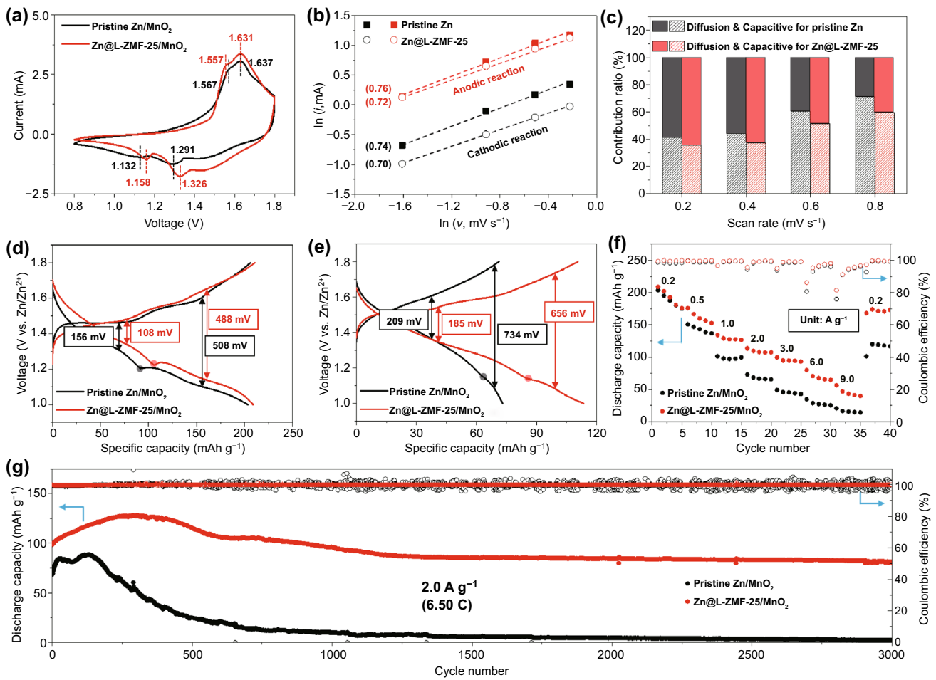
Fig. 4 a Cyclic voltammetry (CV) curves of Zn/MnO 2 full cells at a scan rate of 0.8 mV s -1 . b Linear fitting of ln( i ) as a function of ln( v ) and c contribution ratio of capacitance and diffusion-controlled behaviors for the Zn/MnO 2 full cells with pristine Zn and Zn@L-ZMF-25 anodes. Discharge–charge voltage profiles at current densities of d 0.2 and e 2.0 A g -1 . f Rate performance (unit: A g -1 ) and g capacity retention of the pristine Zn/MnO 2 and Zn@L-ZMF-25/MnO 2 full cells
