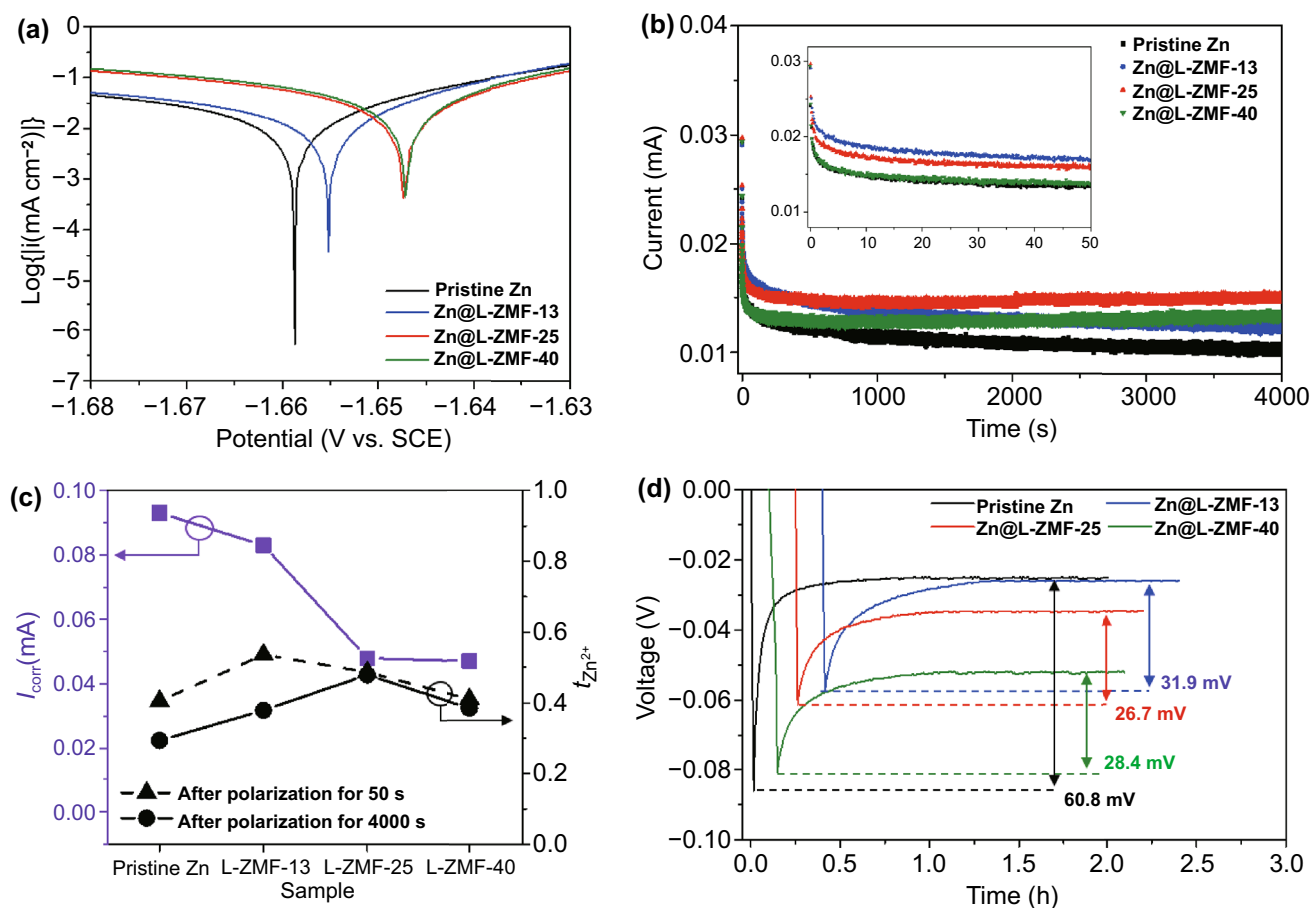
Fig. 2 a Tafel polarization curves and b chronoamperograms of symmetric cells at a constant overpotential of 25 mV. c Summary for the corrosion current and transference number at the 50th and 4000th s. d Nucleation overpotential at a current density of 0.2 \text{ mA cm}^{-2} with an areal capacity of 0.4 \text{ mAh cm}^{-2} for pristine Zn, Zn@L-ZMF-13, Zn@L-ZMF-25, and Zn@L-ZMF-40
