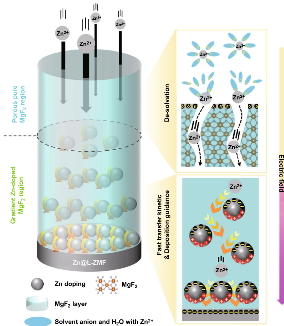
Scheme 1 Illustration of the limitedly Zn-doped MgF 2 thin passivation layer on Zn metal, with a schematic depiction of Zn ion migration through both the porous pure MgF 2 region and gradient Zn-doped MgF 2 region during the Zn ion plating process
