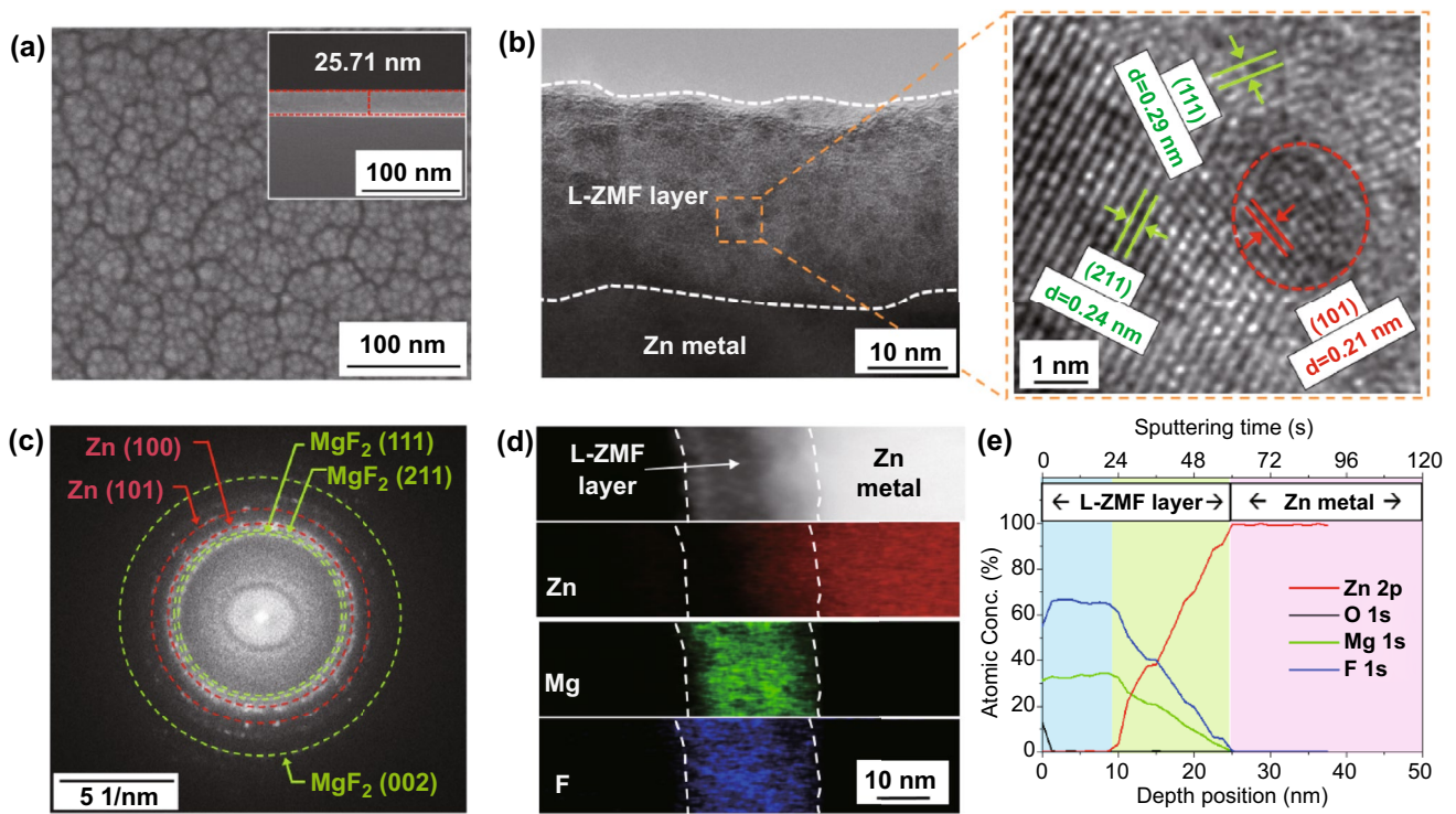
Fig. 1 a Top-view and cross-sectional SEM images of Zn@L-ZMF-25. b Cross-sectional TEM-image and c FFT pattern of the L-ZMF layer of Zn@L-ZMF-25. d Elemental TEM-maps and e depth XPS-profile for Zn@L-ZMF-25.
