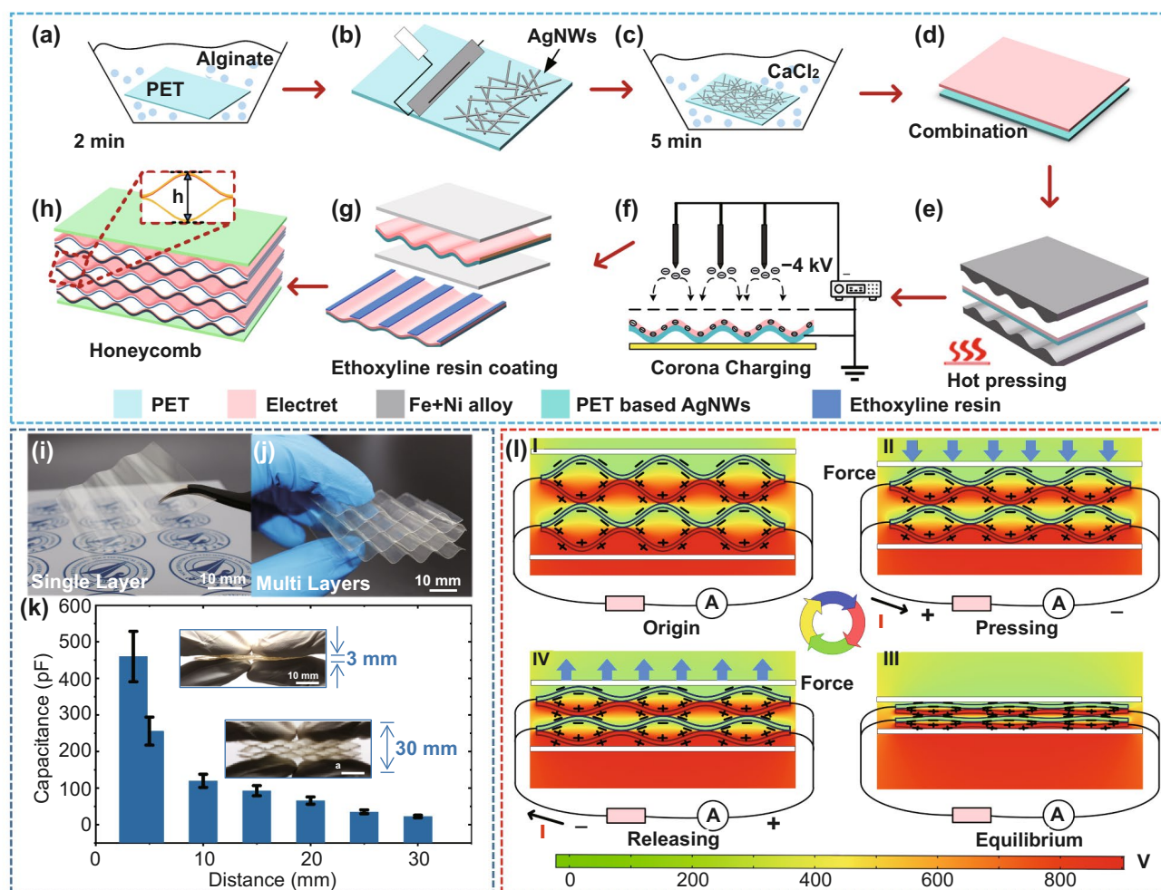
Fig. 2 Fabrication processes and working mechanisms of the proposed h-TENG: a PET thin film is treated with alginate for 2 min. b AgNWs are pressed onto the surface of PET by rolling process. c \text{CaCl}_2 treatment is used to ‘weld’ the AgNWs onto the surface of PET thin film. d FEP electret thin film is bonded onto PET/AgNWs film surface with ethoxylate resin. e A single-wavy structure is formed using iron alloy templates through high-temperature molding process. f A corona discharging process is used to implant charge into FEP electret thin films. g Honeycomb structures are assembled by stacking multilayered PET/AgNWs/FEP composite together. h–j schematic illustration and optical photographs of the fabricated h-TENG device. k Capacitance values change from 20 to 480 pF when the height of h-TENG changes from 3 cm to 3 mm with stacking triple-layer wavy structure. l Electric field and charge redistribution within four stages of h-TENG in a compress-release cycle: I Initial stage of original state. II Electrostatic induction by electrets when two electrodes get close to each other under external compressive force. III Contact triboelectrification when two electrodes get intimate contact with each other. IV Charge flows back when releasing
