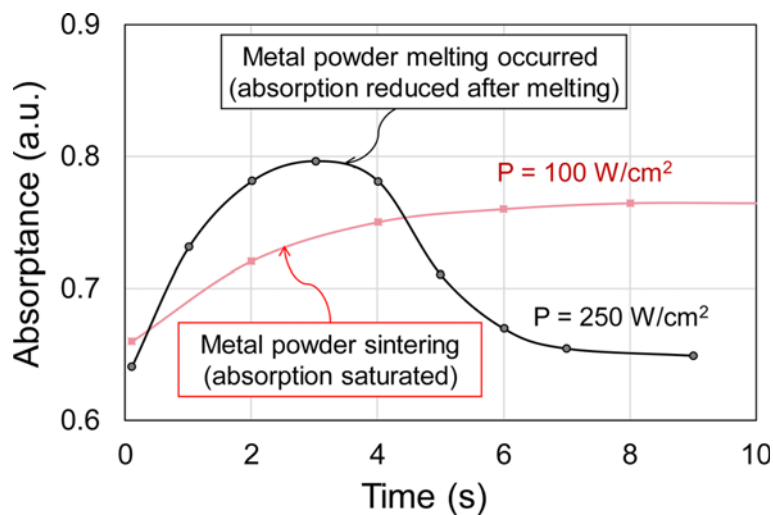
Fig. 15 Variation of absorption of Ni-alloy I metal powder with Nd:YAG laser processing time
