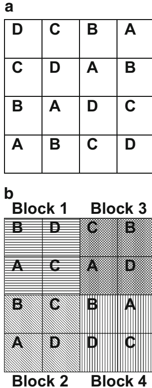
Fig. 1 a Latin square with four treatments or varieties ( A, B, C, D ). In a Latin square, treatments or varieties were replicated only once in each row or column, but the choice among the several arrangements that fulfilled this condition was made at random. Latin squares and randomised blocks were developed by Ronald Fisher with the help of the RES experimental scientists. During the 1920s these arrangements became widely used for the RES annual experiments. b Randomised blocks with four treatments or varieties ( A, B, C, D ). In the scheme there are four 2 \times 2 blocks. Each treatment or variety appeared once in random arrangement in each block, but, unlike the Latin square, the same treatment or variety could be repeated in the same row or column. Randomised blocks were less accurate than Latin squares, but could be used when the number of replications was not equal to the number of treatments or varieties to be tested
