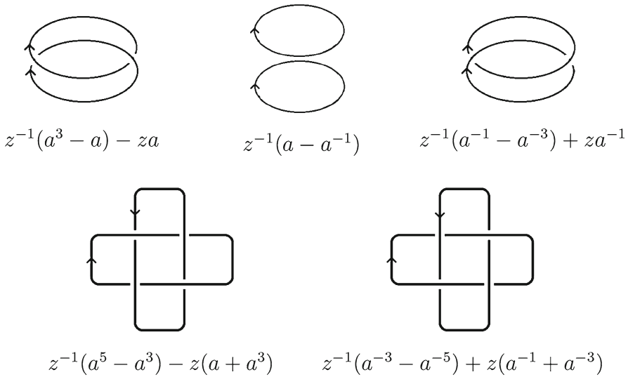
Fig. 7 HOMFLY polynomial of some torus links
