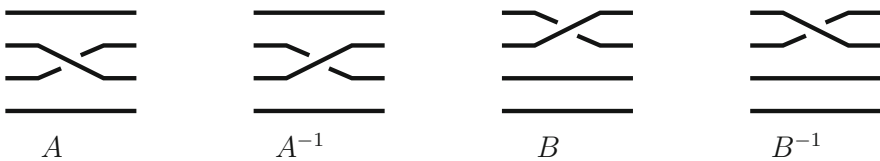
Fig. 1 Fragments of natural diagrams
