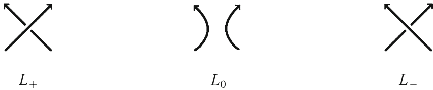
Fig. 5 Outside of these regions the three links coincide
