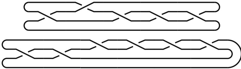
Fig. 3 Two natural diagrams of the table knot 5_2
