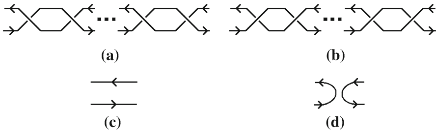
Fig. 6 The differing portions of the links L_n . In the first two pictures the elementary fragment is repeated \frac{|n|}{2} times. a n > 0 . b n < 0 . c n = 0 . d n = \infty
