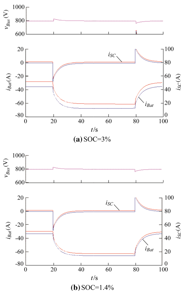
Fig. 13 Dynamic response of supercapacitor and battery current to power fluctuation
