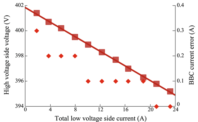
(c) droop curve and current difference
