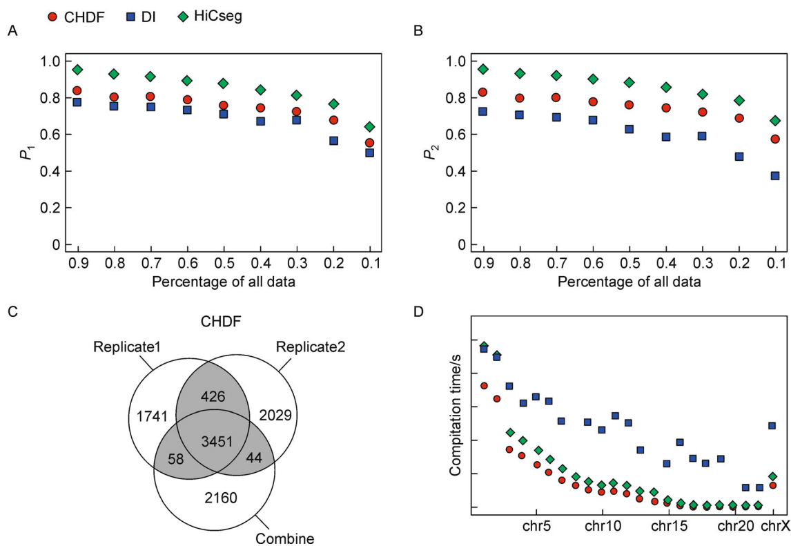
Figure 4. Robustness and time cost of the three methods. (A, B) The robustness to technical noise of three methods was compared by applying three methods to subsampled data in mouse ES cell. Here robustness was measured by two parameters P_1 (A) and P_2 (B). (C) Number of domains called by CHDF in two replicate and combined datasets. The intersection represented the same domains called in different Hi-C datasets. (D) The comparison of computational time cost of three methods in human IMR90 cell line. For the time cost comparison, a single 3.2 GHz CPU was used.
