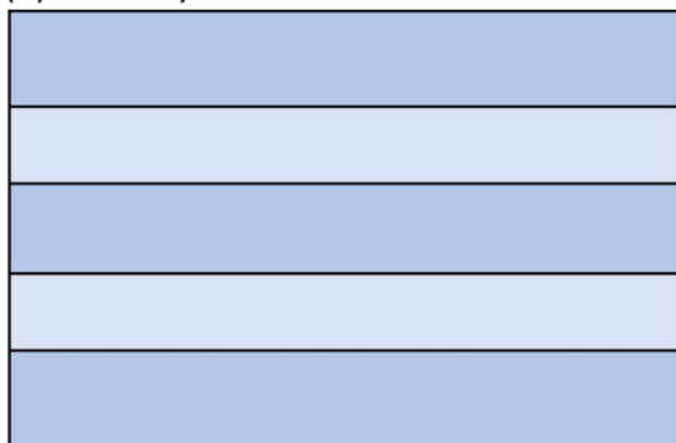
Fig. 10 Schematic representation of grain boundaries in a polycrystalline materials and b multilayered heterostructures. Variations in colors represent different crystallographic orientations in grains or different material compositions in solid solutions or heterostructures. Grain boundaries are denoted with black lines
