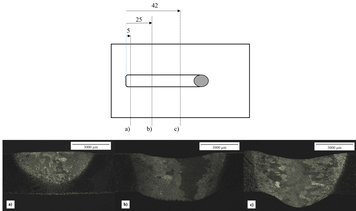
Fig. 3 Weld cross sections showing difference in weld grain structure and weld bead dimensions. The three cross sections are taken from the same test plate but at different locations, a) start of the weld, b) at steady-state condition and c) at area experiencing maximum amount of bending
