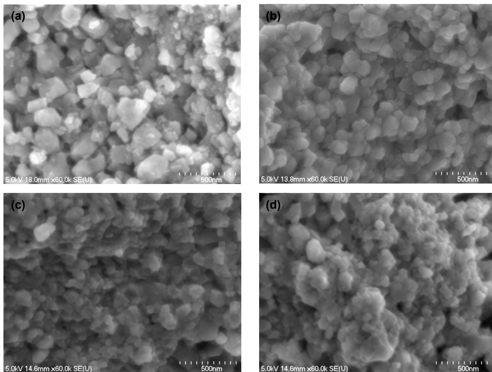
Fig. 2(i) SEM of BST ceramics ball milled for 20 h and sintered at (a) 1200 °C, (b) 1250 °C, (c) 1300 °C and (d) 1350 °C for 2 h.
