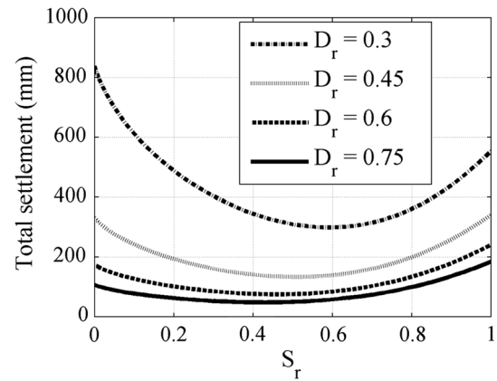
Fig. 2 Predicted settlements of 6.35 m-thick sand layers having different relative densities using the empirical methodology of Ghayoomi et al. [6]
