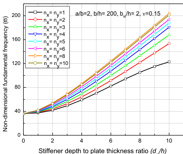
Fig. 20 Variation of the non-dimensional fundamental frequency of eccentric cross-stiffened clamped plate with stiffener depth to plate thickness ratio (case-VI)
