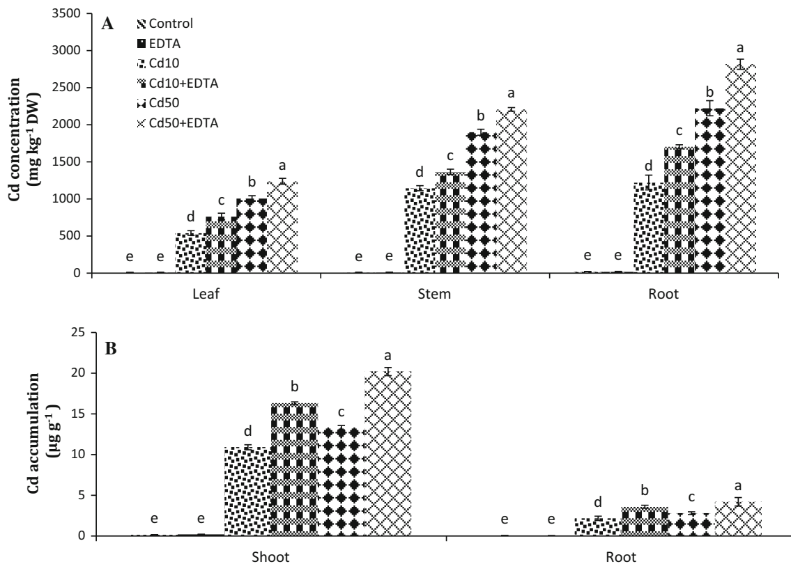
Fig. 4 Cadmium concentration (A) and accumulation (B) in leaf, stem and roots of B. napus seedlings grown in solution culture with different Cd treatments (0, 10 and 50 µM) treated or not with 2.5 mM
