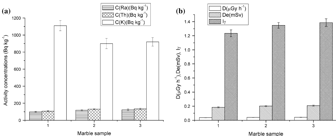
Fig. 4 a Activity concentrations of ^{226}\text{Ra} , ^{232}\text{Th} and ^{40}\text{K} in marble samples, b gamma index, dose rate and annual effective dose for marble samples
