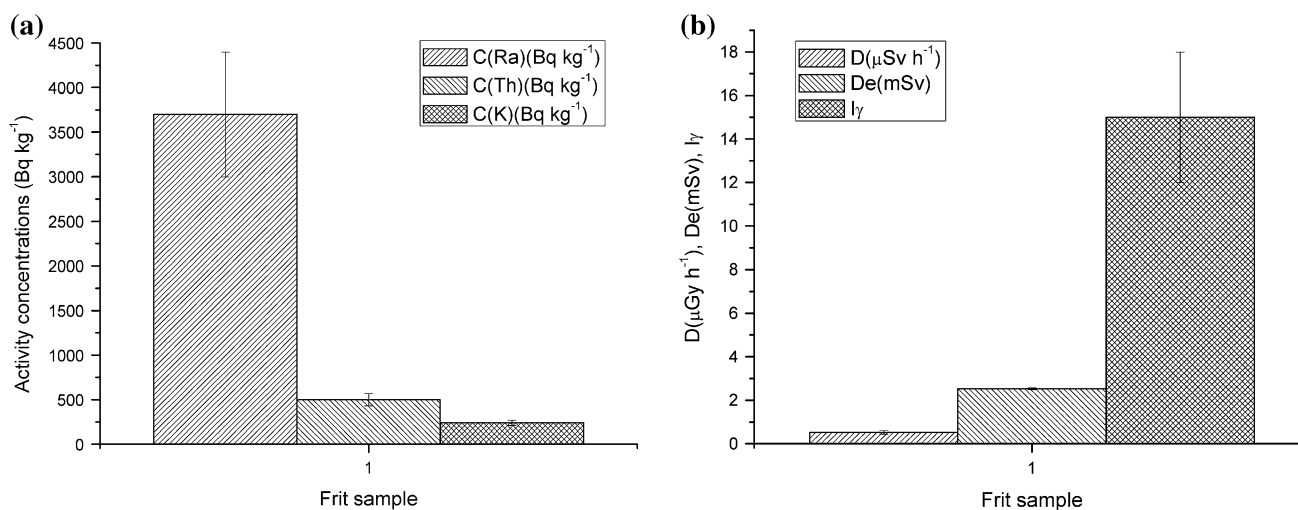
Fig. 9 a Activity concentrations of 226 Ra, 232 Th and 40 K in frit samples, b gamma index, dose rate and annual effective dose for frit samples
