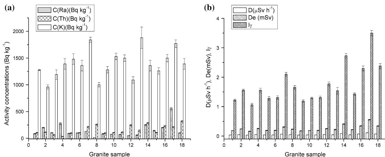
Fig. 3 a Activity concentrations of ^{226}\text{Ra} , ^{232}\text{Th} and ^{40}\text{K} in granite samples, b gamma index, dose rate and annual effective dose for granite samples
