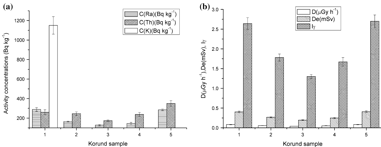
Fig. 8 a Activity concentrations of ^{226}\text{Ra} , ^{232}\text{Th} and ^{40}\text{K} in korund samples, b gamma index, dose rate and annual effective dose for korund samples
