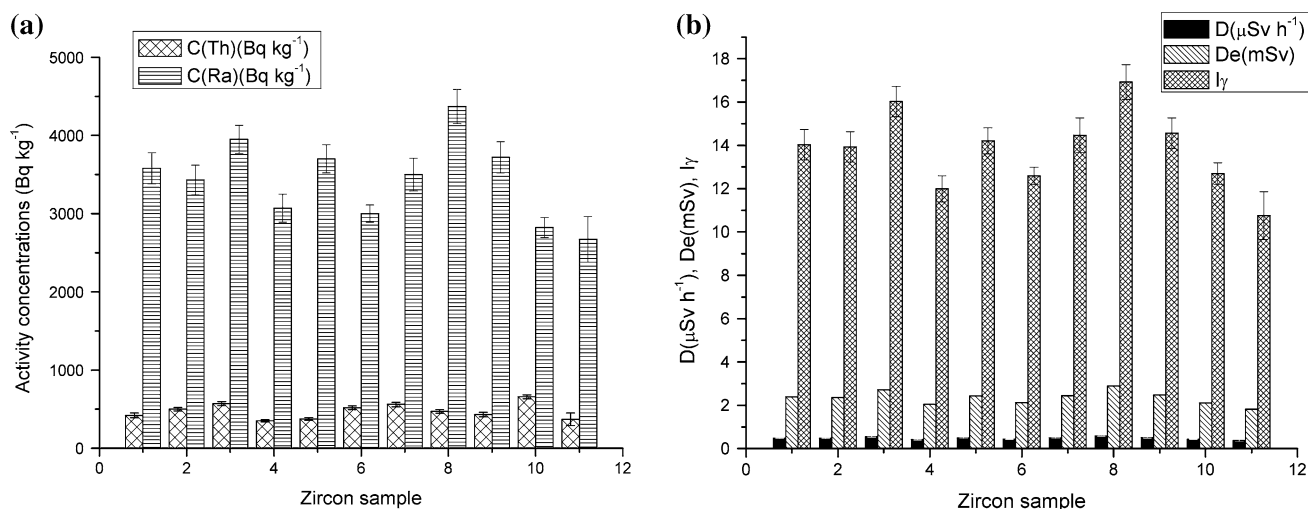
Fig. 2 a Activity concentrations of 226 Ra and 232 Th in zircon samples, b gamma index, dose rate and annual effective dose for zircon samples
