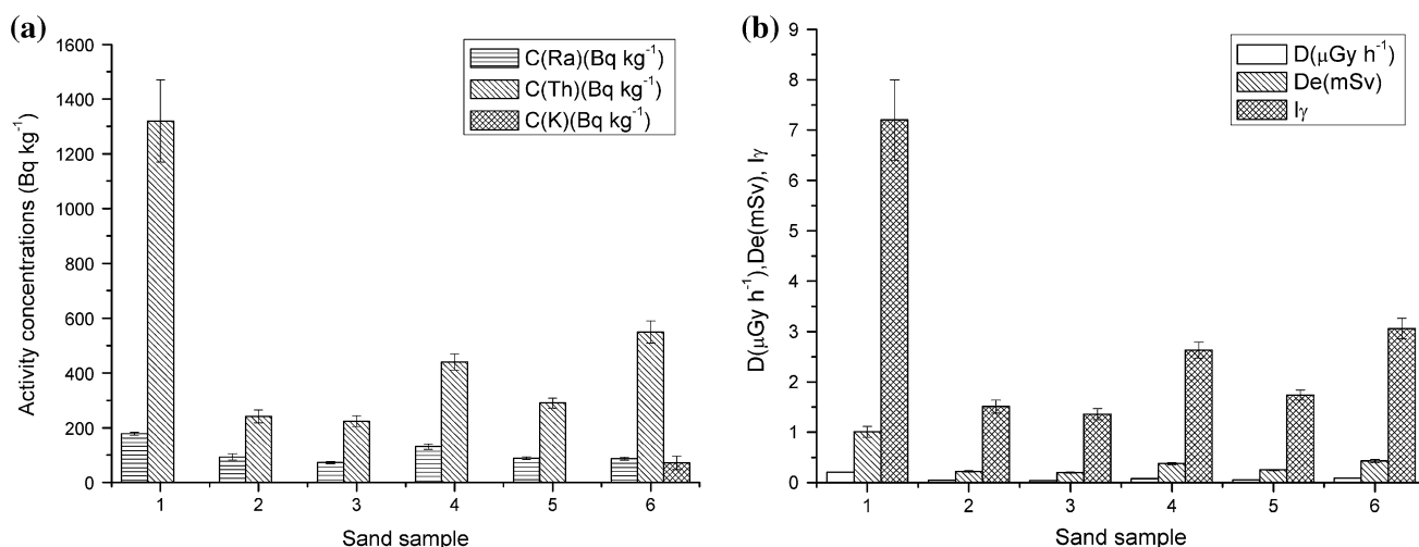
Fig. 5 a Activity concentrations of 226 Ra, 232 Th and 40 K in sand samples, b gamma index, dose rate and annual effective dose for sand samples
