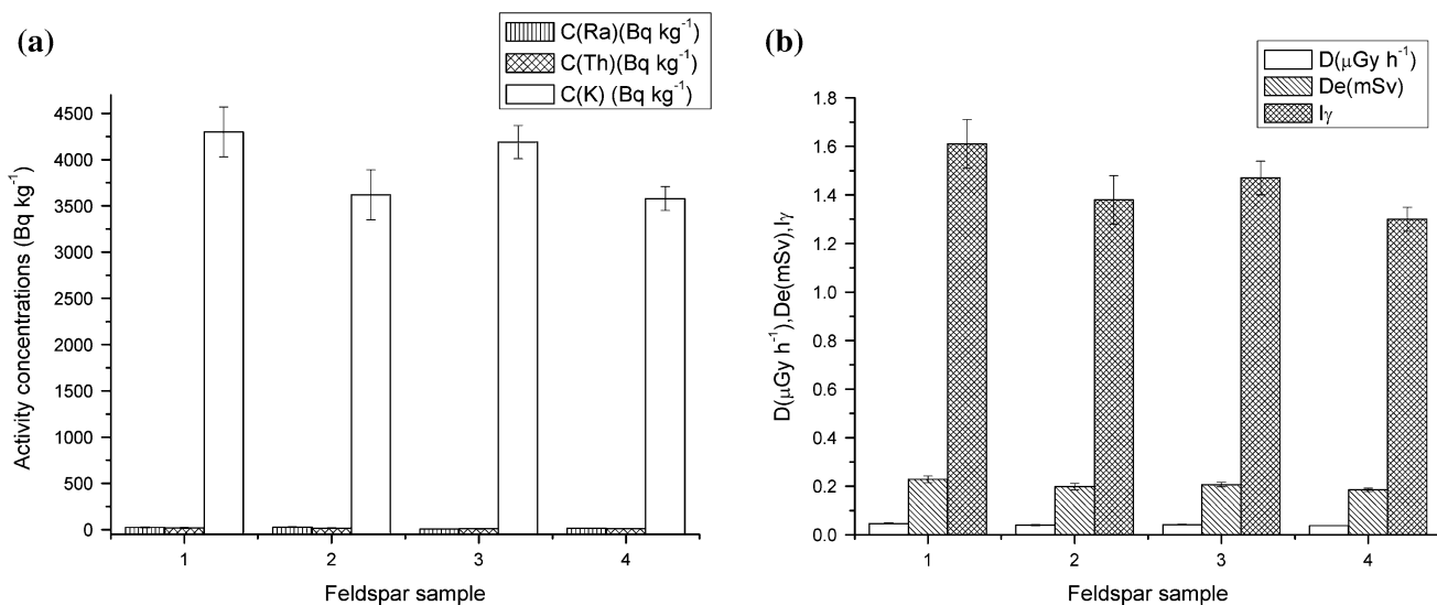
Fig. 7 a Activity concentrations of ^{226}\text{Ra} , ^{232}\text{Th} and ^{40}\text{K} in feldspar samples, b gamma index, dose rate and annual effective dose for feldspar samples
