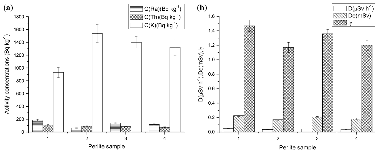
Fig. 6 a Activity concentrations of 226 Ra, 232 Th and 40 K in perlite samples, b gamma index, dose rate and annual effective dose for perlite samples
