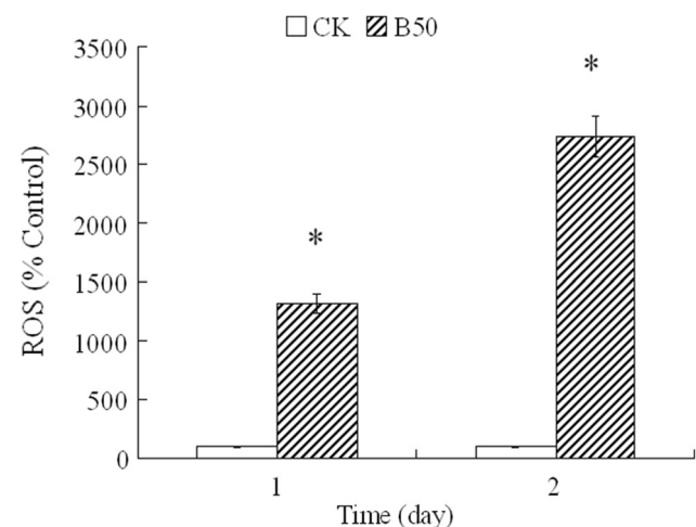
Fig. 6 Effects of inoculation ( 1.9 \times 10^7 cfu/mL) of algicidal bacterium Bacillus sp. B50 on intracellular ROS levels of M. aeruginosa NIES-843. B50: Bacillus sp. B50 inoculation; CK: Control check. Average values \pm standard deviation ( n = 3 ). * p < 0.05
