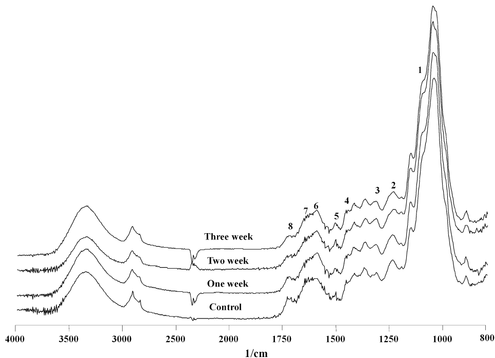
Fig. 2 FTIR spectrum of Streptomyces viridosporus T7A bio-degraded wheat straw for 3 weeks
