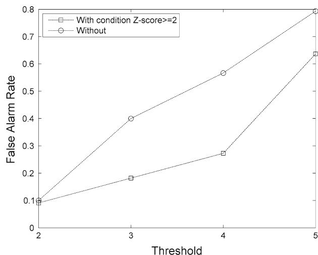
Fig. 8 Effect of condition z -score \geq 2 on false alarm rate
