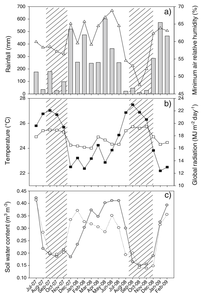
Fig. 1 Seasonal variations in climatic variables over the study period. a Monthly sum of rainfall (bars) and mean of daily minimum air relative humidity (open triangle), b monthly sum of global radiation (closed squares) and mean of air temperature (open squares), and c surface soil water content (SWC) in Terra Firme forest (TFF, open circles) and seasonal flooded forest (SFF, gray circles) at 20 cm. The hatched areas correspond to the long dry seasons in 2007 and 2008
