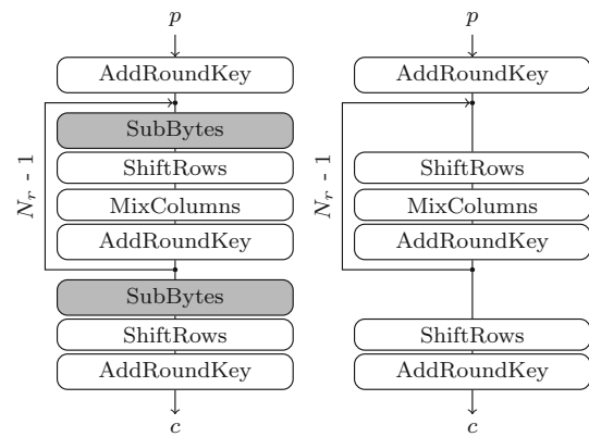
Fig. 10 Comparison between AES (left) and modified \widetilde{AES} (right)
