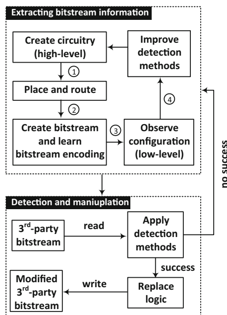
Fig. 2 Strategy of partially replacing an FPGA configuration
