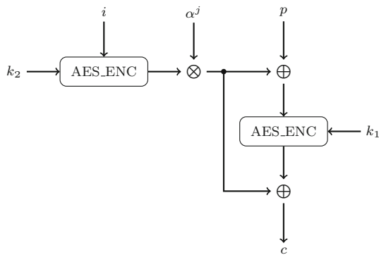
Fig. 9 XTS-AES encryption block digram overview
