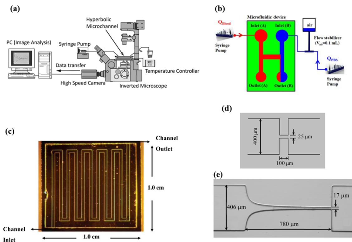
Fig. 5. (Color online) Microfluidic devices employed in blood rheological measurements. (a) The experimental set-up is typically composed of an inverted microscope on which the microfluidic chip is placed, a digital camera for recording images, a syringe pump for imposing a flow rate and a temperature controller for controlling the temperature of the fluid. Reprinted with permission from Yaginuma et al. (2013) (b) Microfluidic analogue of Wheatstone-bridge channel used by Kang and Lee (2013). Reprinted with permission from Kang and Lee (2013). Blood is fed to inlet A and a PBS solution to inlet B by means of syringe pumps. To ensure constant flow rates for both fluids, a flow stabilizer with 0.1 ml cavity volume was placed between the syringe pump and the channel inlet of PBS solution. (c) Microfabricated viscometer used by Srivastava et al. (2005). The channel, 340 \mu\text{m} wide and 36 \mu\text{m} in depth, is etched in glass and bounded to silicon and open to the atmosphere on the inlet and outlet. Reprinted with permission from Srivastava et al. (2005). Copyright (2015) American Chemical Society. (d) Sketch of the microfluidic channel composed of an abrupt contraction followed by an abrupt expansion used by Brust et al. (2013). The depth of the channel is 50 \mu\text{m} . (e) Optical micrograph of the hyperbolic-shaped contraction followed by an abrupt expansion channel similar to that employed by Yaginuma et al. (2013). The depth of the channel is 60 \mu\text{m} . The same type of contraction was also used in the work of Lee et al. (2009) for investigating RBC deformability.
