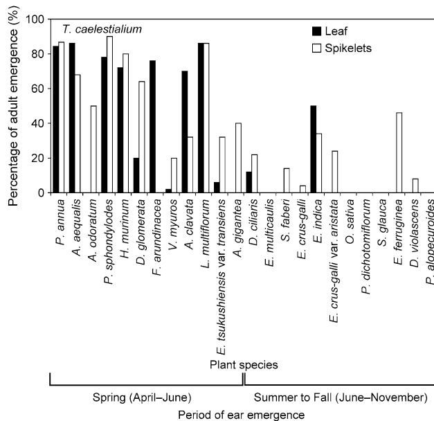
Fig. 2 The percentage of Trigonotylus caelestialium adults that emerged on poaceous plants. We reared 50 nymphs, individually, on the leaves or spikelets of each plant. The names of the plants are listed from left to right in relation to the time of the plant ear appearance
