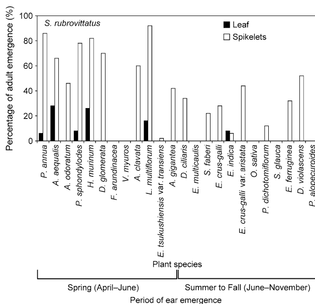
Fig. 3 The percentage of Stenotylus rubrovittatus adults that emerged on poaceous plants. We reared 50 nymphs, individually, on the leaves or spikelets of each plant. The names of the plants are listed from left to right in relation to the time of the plant ear appearance
