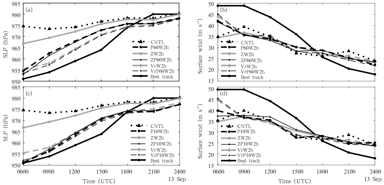
Fig. 8. Forecast (a, c) minimum sea level pressures and (b, d) surface maximum wind with time, compared to the observed best track and CNTL.
