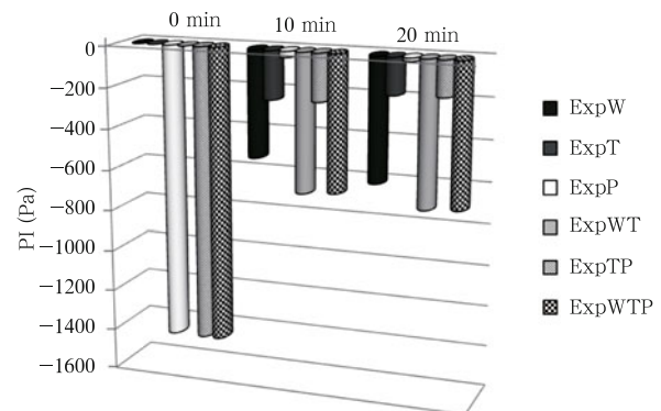
Fig. 7. Pressure impact index (PI; Pa) with time for experiments updating various model variables.
