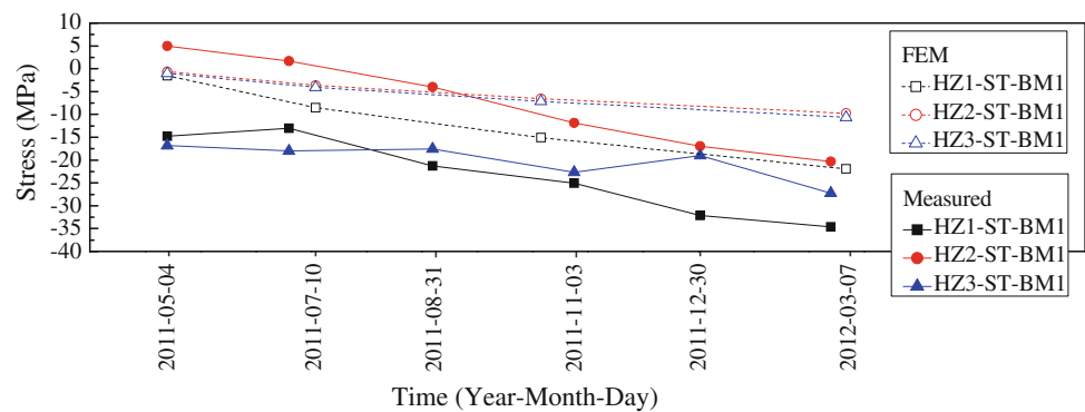
Fig. 16 Stress evolution at different construction stages at the 5th floor
