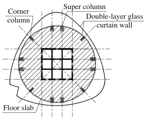
Fig. 5 Standard floor plan of the Shanghai Tower
