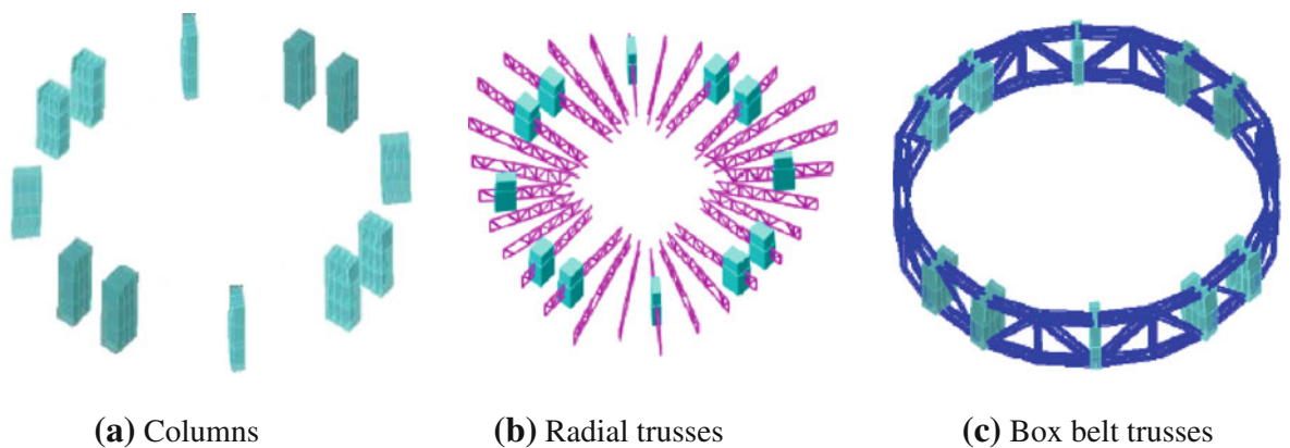
Fig. 4 Components of the mega-frame
