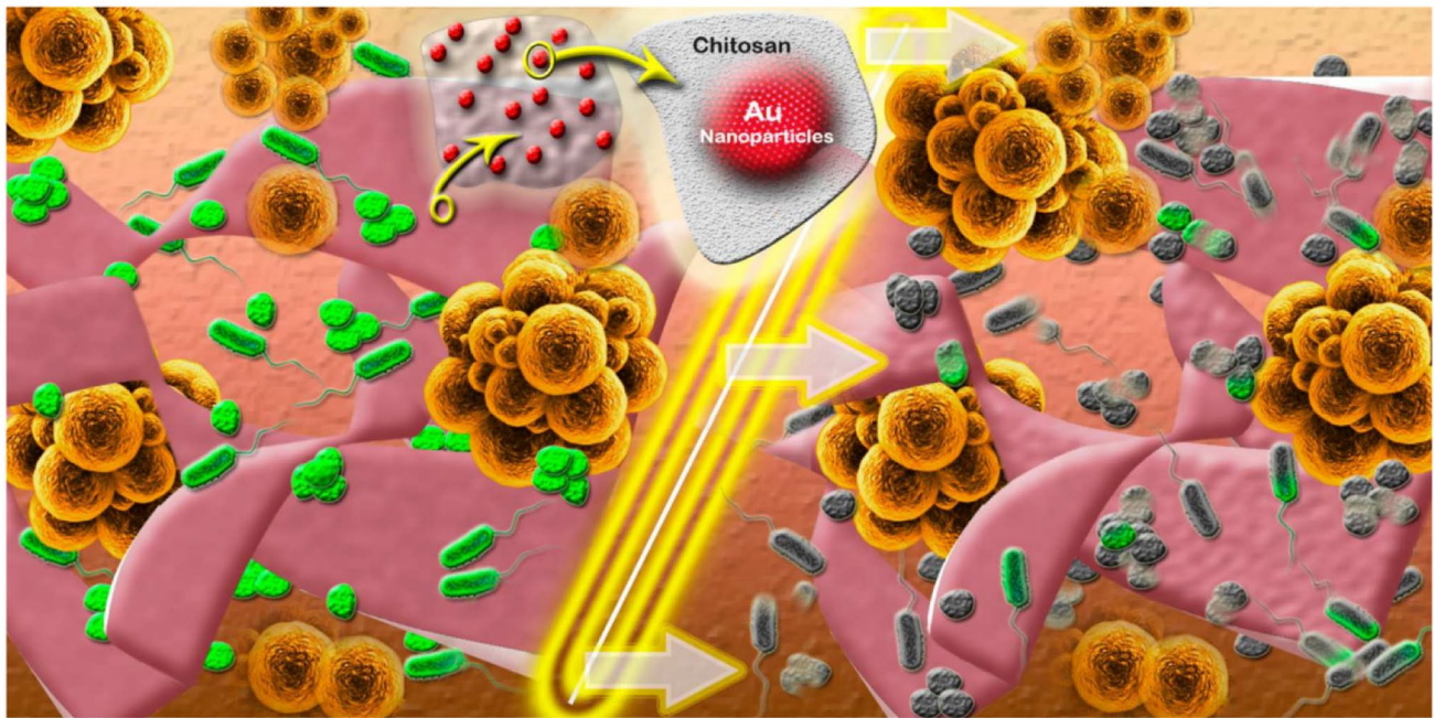
Fig. 1 Schematic diagram of chitosan-gold nanoparticles as efficient antibacterial materials [29]. Copyright © 2014 American Chemical Society
