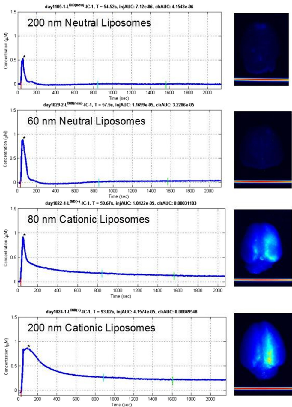
Fig. 3 Dynamics of brain liposomal uptake in healthy rats. Concentration-time curves show the real-time, in vivo uptake of liposomes after ipsilateral carotid artery injection ( left panel ). Multispectral images (MSI) of harvested brain show the degree of liposome deposition for the four liposome types tested ( right panel ). Note that only minimal neutral liposome deposition is observed on postmortem MSI. Higher-intensity MSI signal is evident after 200-nm cationic liposome delivery than after 80-nm cationic liposome delivery
