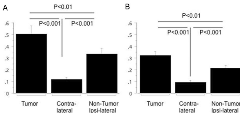
Fig. 5 Delivery efficiency of liposomes to gliomas is size dependent. Bar graphs of tissue concentration after 200-nm (a) and 80-nm (b) liposome delivery are shown. Liposome concentrations were significantly greater in the tumor-bearing region as compared to the contralateral hemisphere
