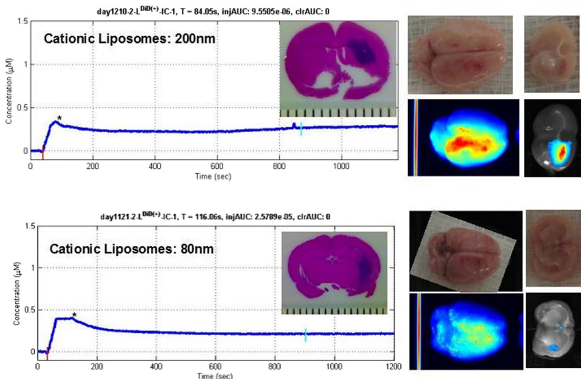
Fig. 4 Cationic liposomes specifically target tumor site. Concentration-time curves ( left panel ) as well as postmortem multispectral imaging (MSI) of intact glioma-bearing brains ( middle panel ) indicate that hemispheric delivery of both large and small cationic liposomes occurs
