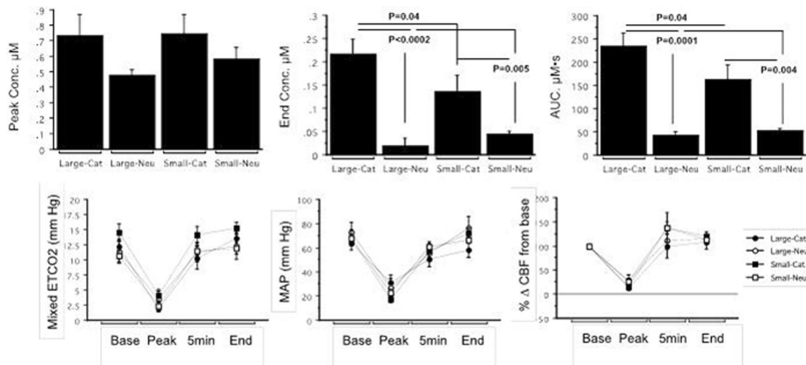
Fig. 2 Hemodynamic changes and liposome delivery after intraarterial injection during transient cerebral hypoperfusion in healthy animals. In vivo measurements of liposome delivery to the ipsilateral hemisphere show that both the end concentration and total tissue exposure (AUC) were significantly highest for large cationic liposomes ( top panel ).
