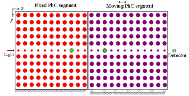
Fig. 1 Layout of the micro-displacement sensor based on the high sensitivity photonic crystal.
