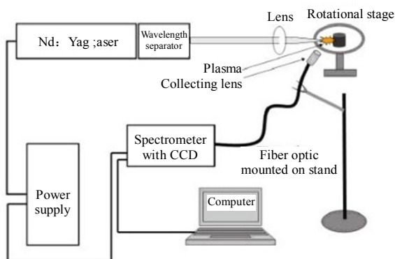
Fig.1 Experimental setup of the LIBS system.
