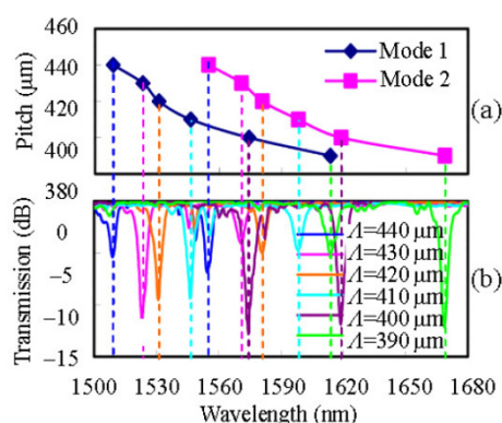
Fig. 7 Transmission spectra of LPFGs written in air-core PBFs: (a) the relationship between the pitch of each LPFG and the corresponding resonant wavelength, and (b) transmission spectra of six LPFGs with different grating pitches, where two attenuation dips for each LPFG are observed from 1500 nm to 1680 nm, indicating that the fundamental mode is coupled to two different higher order modes [42].
