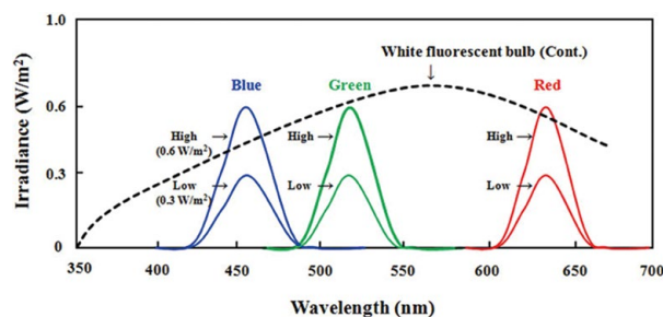
Figure 1. Spectral profiles of light-emitting diodes (LEDs; blue, 450 nm; green, 520 nm; red, 640 nm) and white fluorescent bulb (Cont.) used in the present study. Two different intensities were used (low, 0.3 W/m^2 ; high, 0.6 W/m^2 ) for each LED treatment.
