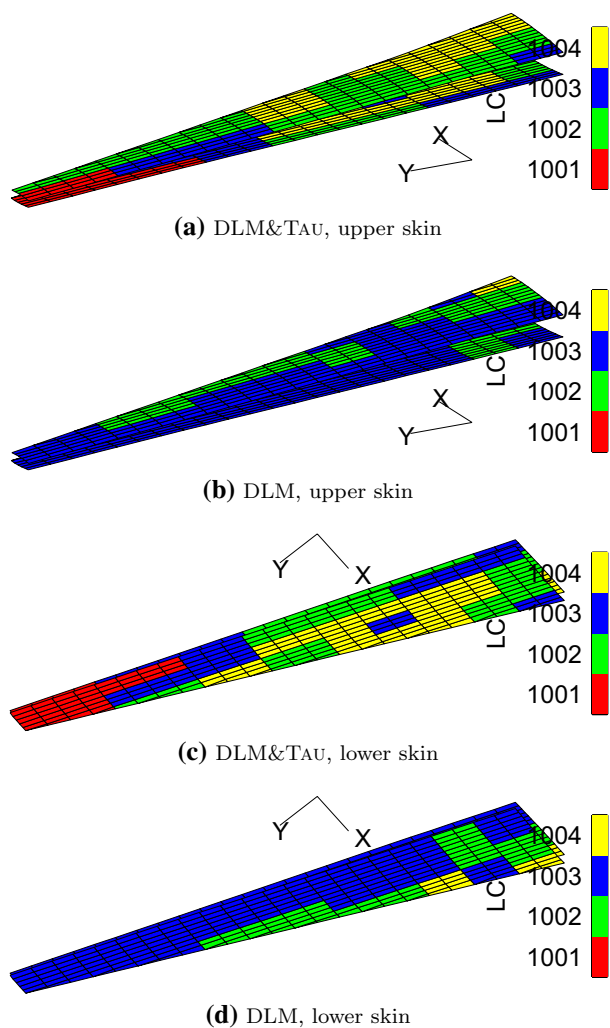
Fig. 14 Optimized design, sizing load case per field, unbalanced laminates
