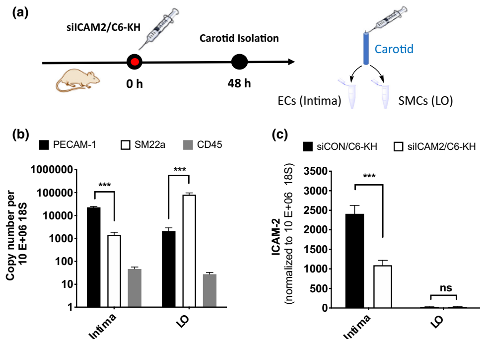
FIGURE 5. Efficient in vivo ICAM2 knockdown in the endothelium when siCAM2 was delivered using C6-KH polymer. (a) siCAM2-C6-KH and siCON-C6-KH were injected at 2 mg/kg in mice. Two days post-injection, endothelial-enriched (intima) and SMC-enriched fraction (leftover) RNAs were prepared and analyzed by qPCR for gene expression. (b) As a quality control, expression of markers of ECs (PECAM-1), medial SMCs (SM22a), and leukocytes (CD45) were determined, whereas (c) ICAM2 expression was analyzed by RT-qPCR. n = 5 , mean \pm SEM; *** p < 0.001 .
