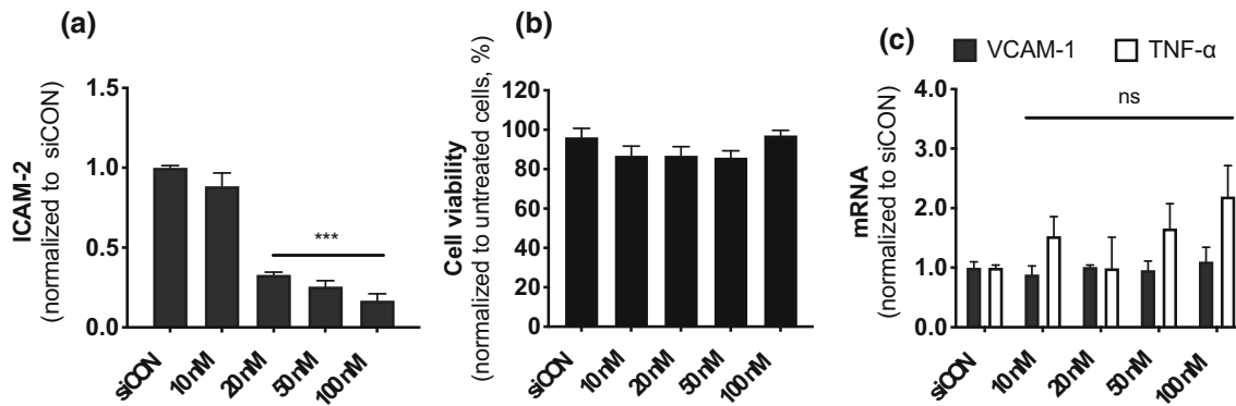
FIGURE 4. Efficient ICAM2 knockdown in iMAECs. iMAECs were transfected with an increasing concentration of siCAM2 encapsulated with C6-KH. (a) ICAM2 expression was determined 48 h post-transfection by RT-qPCR, (b) cell viability of iMAECs were determined by the MTS assay, and (c) VCAM1 and TNF- \alpha expression was analyzed by qPCR. n = 4 , mean \pm SEM; *** p < 0.001 .
