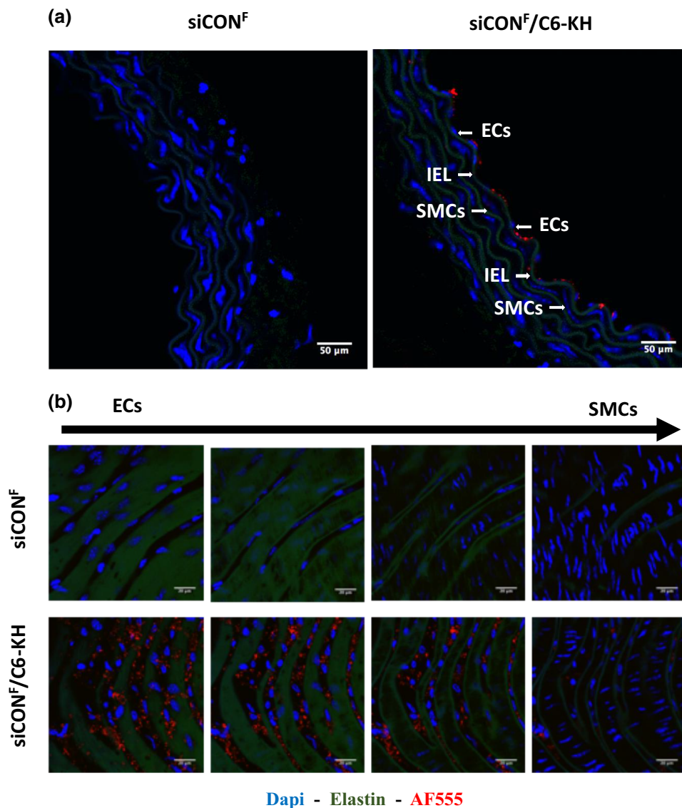
FIGURE 3. siCONF F delivery to endothelial layer. Abdominal aortas of C57Bl6 mice were dissected out and incubated ex vivo with siCONF F -C6-KH or naked siCONF F for 1 h, followed by either frozen cross-section (a) or en face (b) imaging by confocal microscopy. Blue DAPI for nuclear, Green auto-fluorescence for elastic laminae, Red AF555 for siCONF F are shown.
