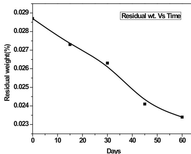
Fig. 1 Change in residual weight of HDPE with incubation time. The graph shows that there is regular decrease in weight during incubation of HDPE film with K. Pneumoniae . Values represent the average of three independent experiments. Error bars indicate standard deviation ( \pm SD). Statistical significance between the groups was evaluated at p = 0.05 significance level
