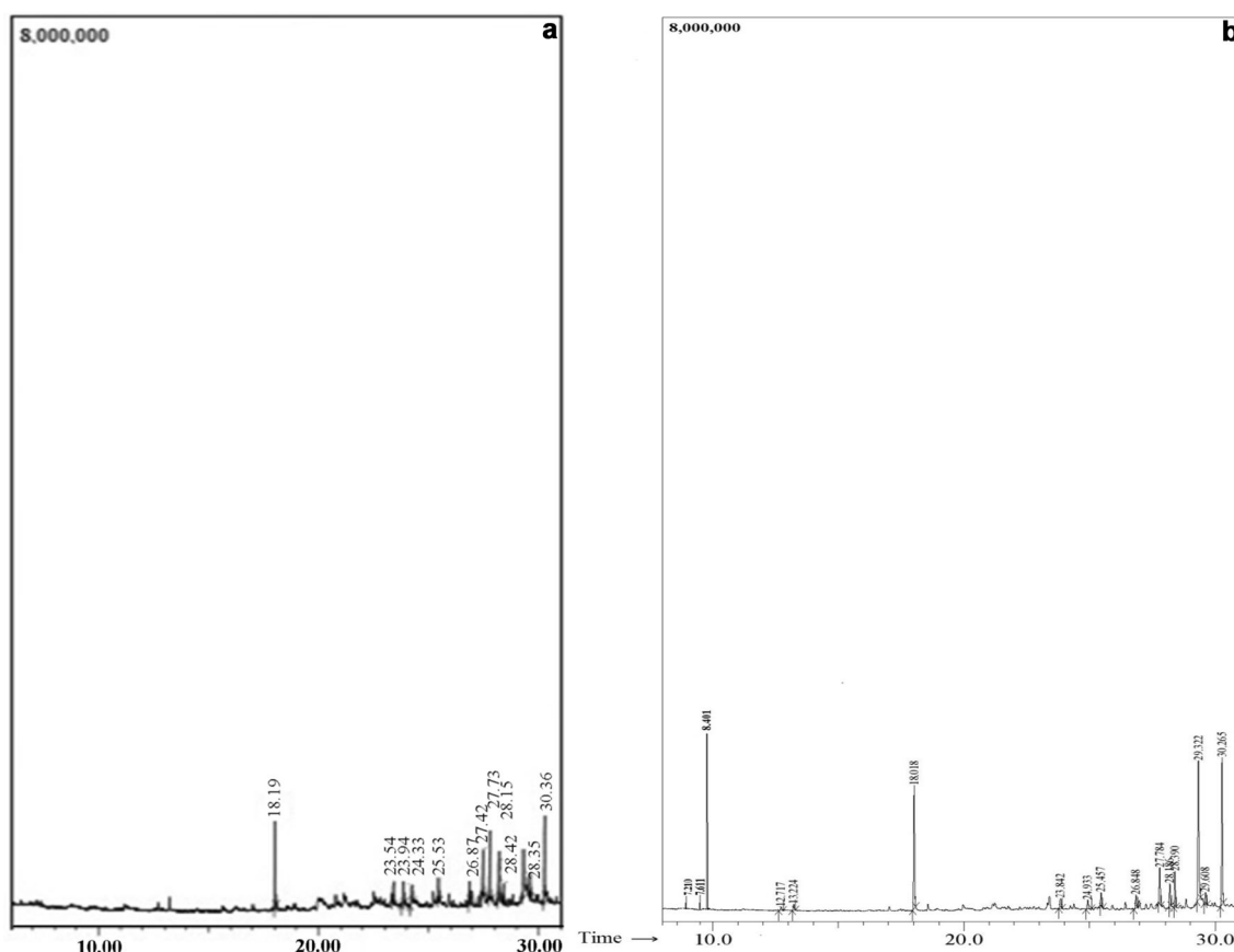
Fig. 7 Note It is clear in Fig. 7a that GC–MS of control HDPE film is different from the treated HDPE film which has various monomers, acidic compounds, and oxidized compounds which are present at less retention time after biodegradation
