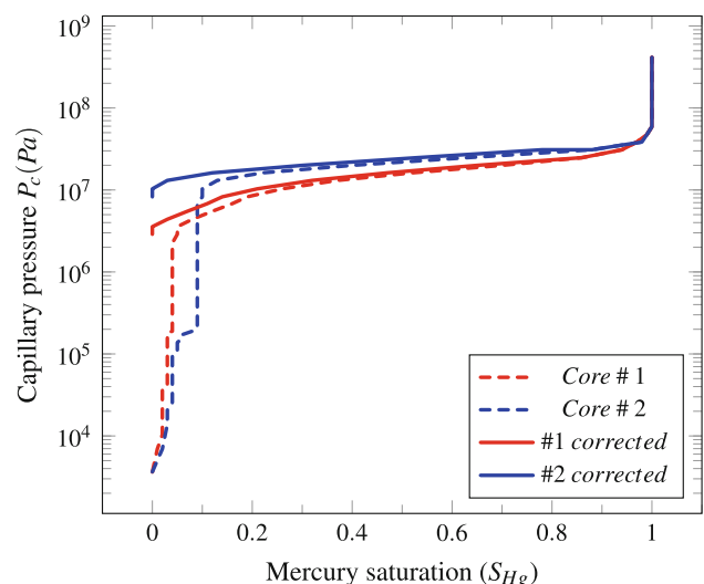
Fig. 6 Plots of capillary pressure versus mercury saturation for the carbonate core samples 1 and 2. The red and blue colours represent vertically and horizontally obtained samples, respectively. The dash and thick lines represent the uncorrected and conformance corrected data, respectively
