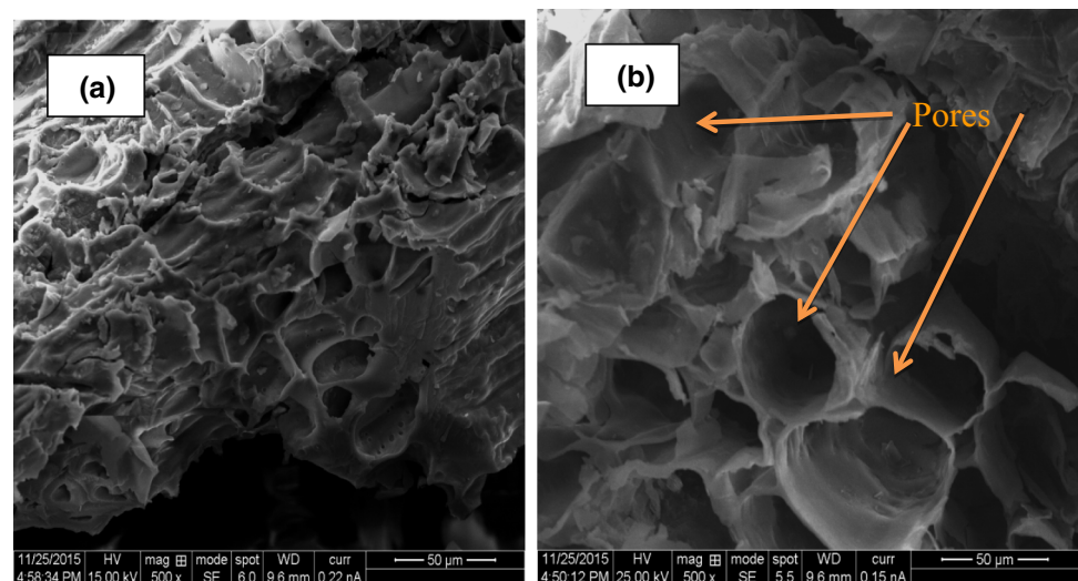
Fig. 2 SEM images of a CHR (Mag \times 500 ) and b CHA (Mag \times 500 )
