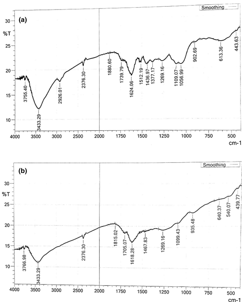
Fig. 1 FTIR spectra of a raw coconut husk (RCH) and b activated coconut husk (CHA)
