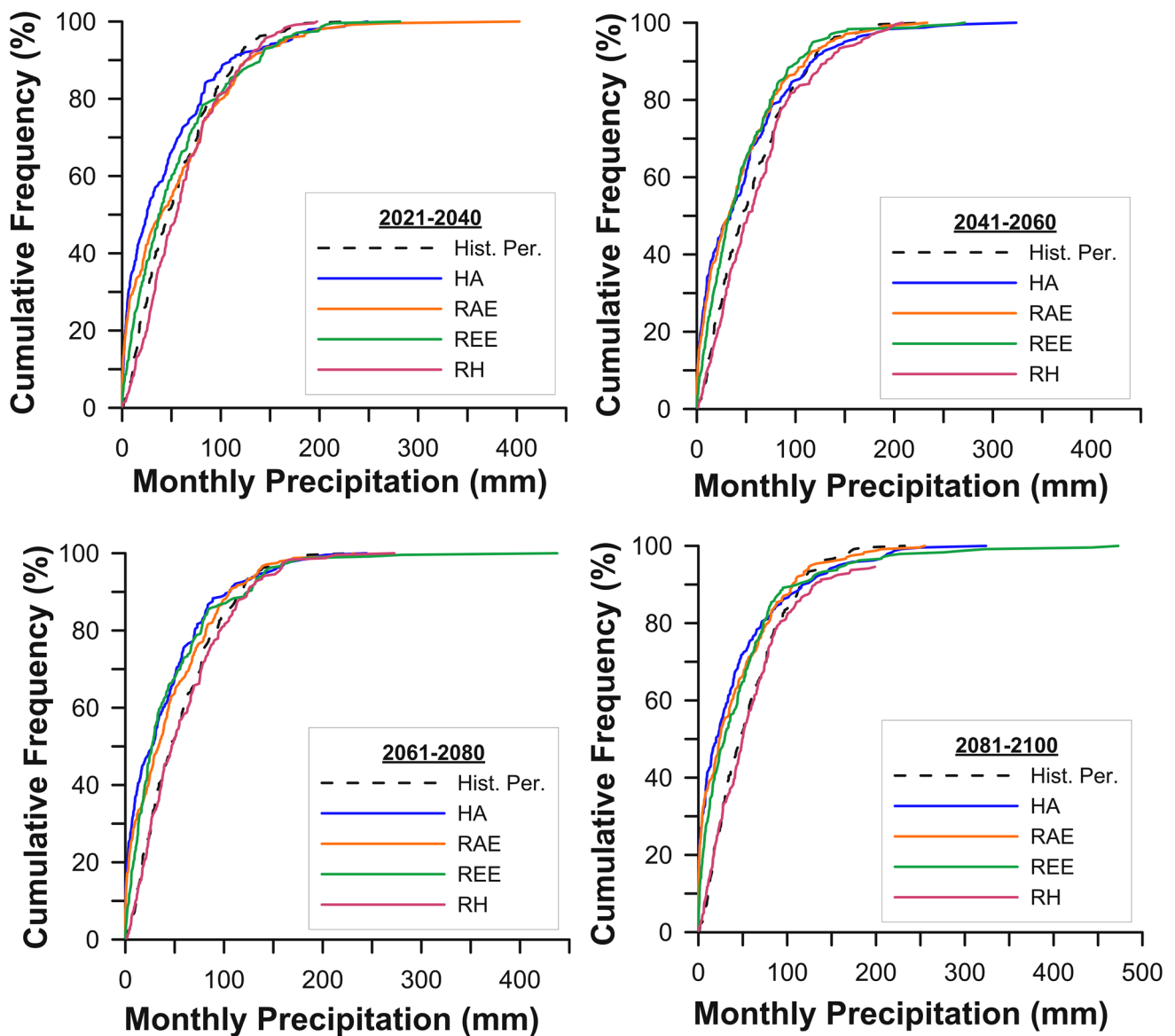
Fig. 6 Cumulative frequency diagrams of monthly precipitation for the historical period (1981–2000) and all RCM–GCM combinations at the four sub-periods
