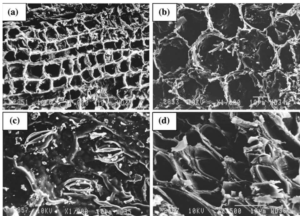
Fig. 4 SEM images of PDLP a before adsorption, b after adsorption of Cr(VI), c after adsorption of Ni(II) and d after adsorption of Cu(II)
