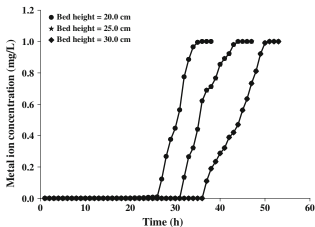
Fig. 10 Breakthrough curves for biosorption of Cr(VI), Ni(II) and Cu(II) from electroplating waste water at different bed heights (flow rate = 2.0 mL min -1 , pH = 4.5.)
