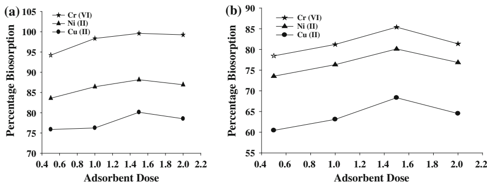
Fig. 7 Effect of adsorbent dose on Cr(VI), Ni(II) and Cu(II) biosorption on a SCLP and b PDLP (initial metal ion concentration = 50 mg L -1 , pH = 2.0 for Cr(VI), 6.0 for Ni(II) and 4.0 for Cu(II), contact time = 12 h, rpm = 225 at 30 °C)
