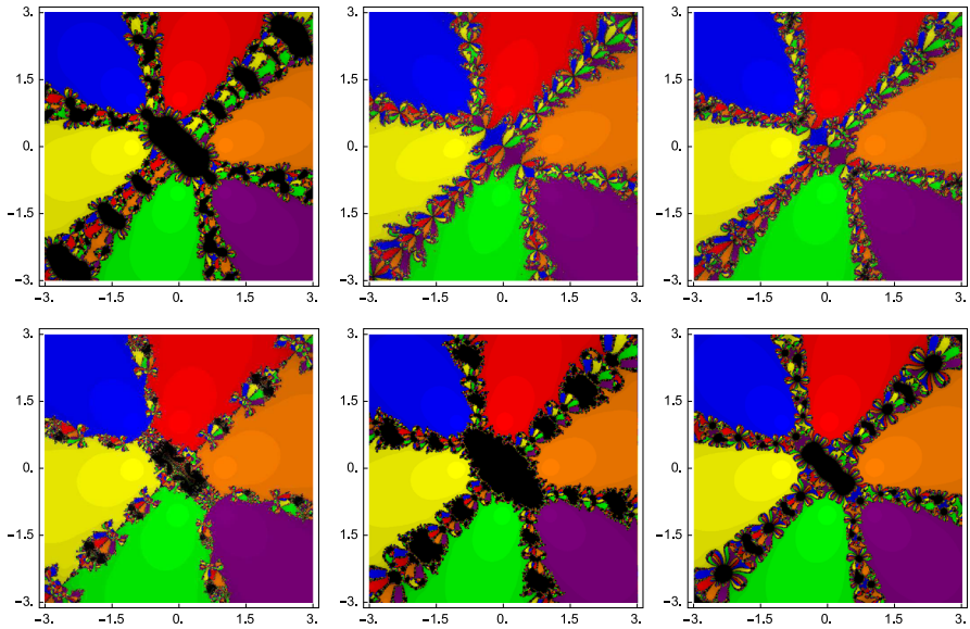
Fig. 4 Comparison of basins of attraction of methods MSSV, CL, N ( top row, left to right ), and SS, BCST, TP ( bottom row, left to right ) for the test problem p_4(z) = (z^4 - 1)(z^2 + 2i) = 0
