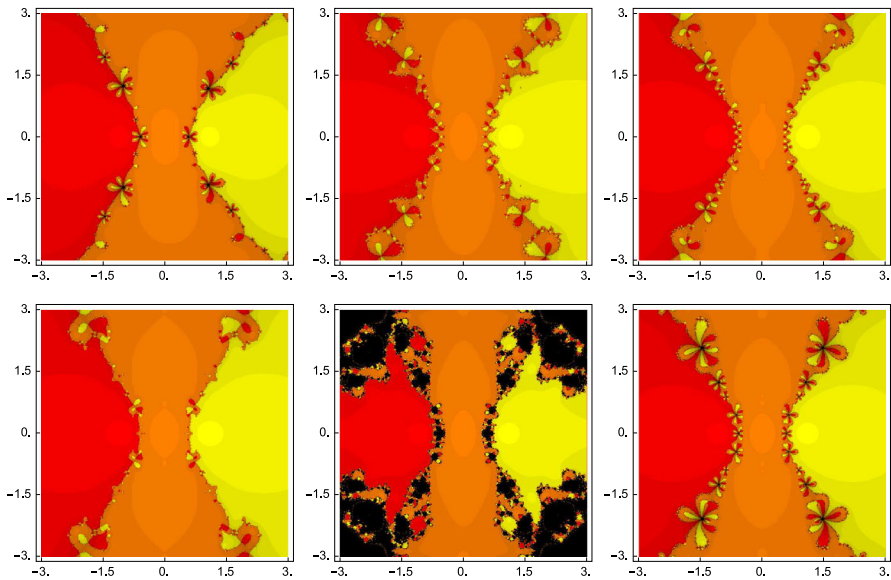
Fig. 2 Comparison of basins of attraction of methods MSSV, CL, N (top row, left to right), and SS, BCST, TP (bottom row, left to right) for the test problem p_2(z) = z^3 - z = 0
