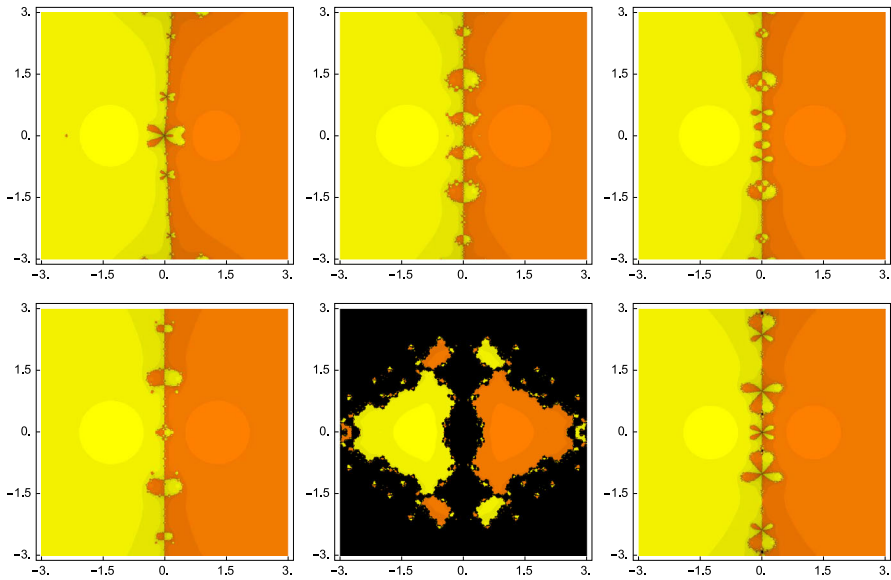
Fig. 1 Comparison of basins of attraction of methods MSSV, CL, N (top row, left to right), and SS, BCST, TP (bottom row, left to right) for the test problem p_1(z) = z^2 - 1 = 0
