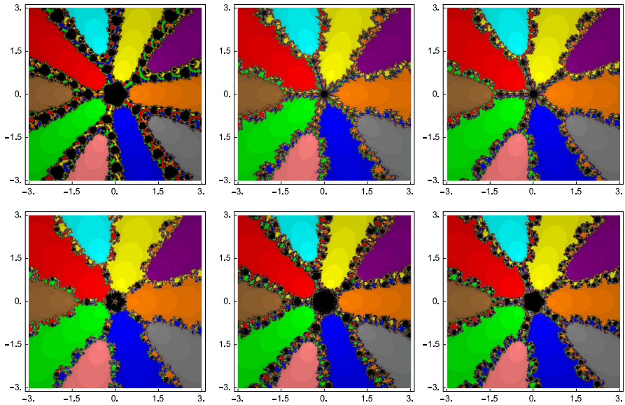
Fig. 6 Comparison of basins of attraction of methods MSSV, CL, N (top row, left to right), and SS, BCST, TP (bottom row, left to right) for the test problem p_6(z) = (10z^5 - 1)(z^5 + 10) = 0
