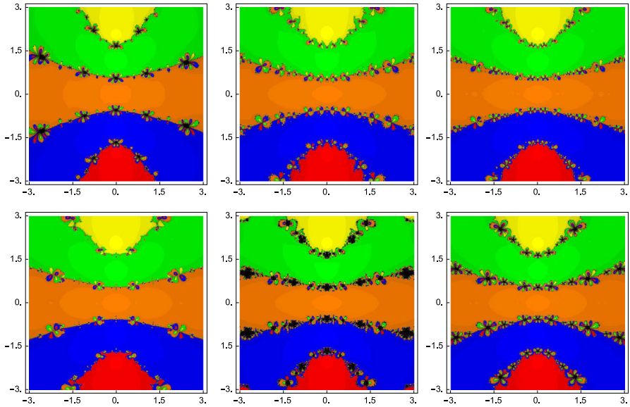
Fig. 3 Comparison of basins of attraction of methods MSSV, CL, N ( top row, left to right ), and SS, BCST, TP ( bottom row, left to right ) for the test problem p_3(z) = z(z^2 + 1)(z^2 + 4) = 0
