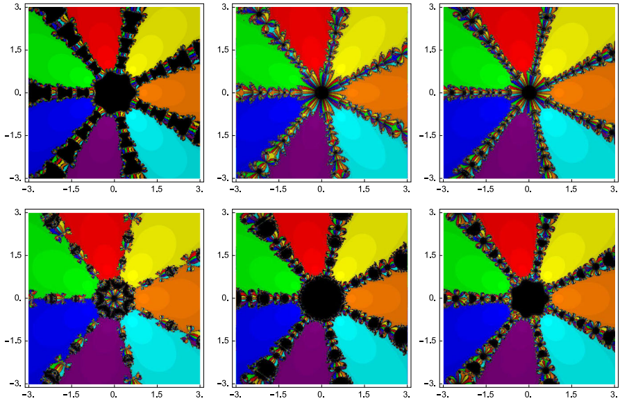
Fig. 5 Comparison of basins of attraction of methods MSSV, CL, N (top row, left to right), and SS, BCST, TP (bottom row, left to right) for the test problem p_5(z) = z^7 - 1 = 0
