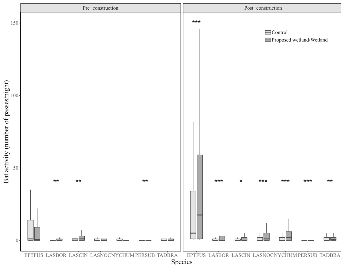
Fig. 2 Species specific bat activity (number of passes per night) in control and proposed wetland sites before the wetland construction (November 19th, 2016–March 14th, 2017) and in control and wetland sites after the construction (March 15th, 2017–March 28th, 2018) at the University of North Carolina Greensboro. Species abbreviations are: ( Eptesicus fuscus (EPTFUS), Lasiurus borealis (LASBOR), Lasiurus cinereus (LASCIN), Lasionycteris noctivagans (LASNOC), Nycticeius humeralis
