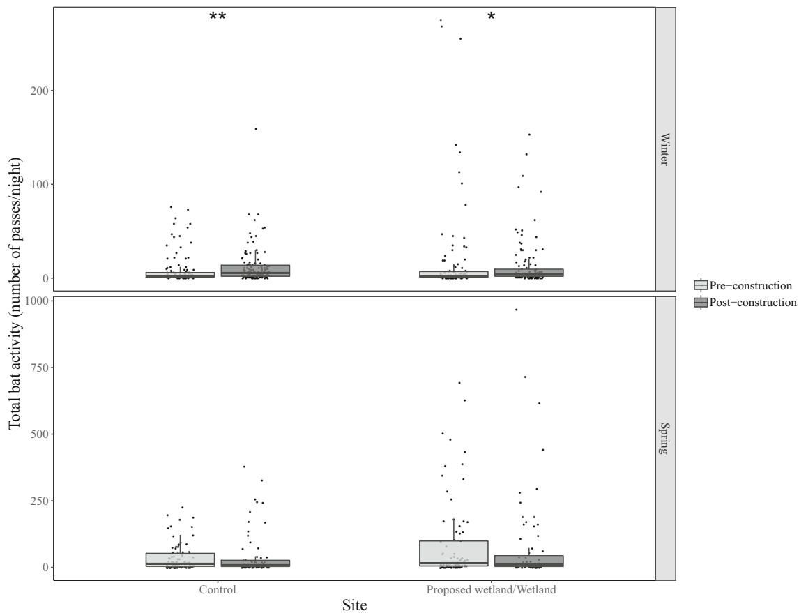
Fig. 3 Total bat activity (number of passes per night) in control and proposed wetland sites before the wetland construction in the Winter (November 19th, 2016–January 31st, 2017) and Spring (February 1st, 2017–March 14th, 2017), and in control and wetland sites after the construction in the Winter (November 19th, 2017–January 31st, 2018) and Spring (February 1st, 2018–March 14th, 2018) at the University of North
