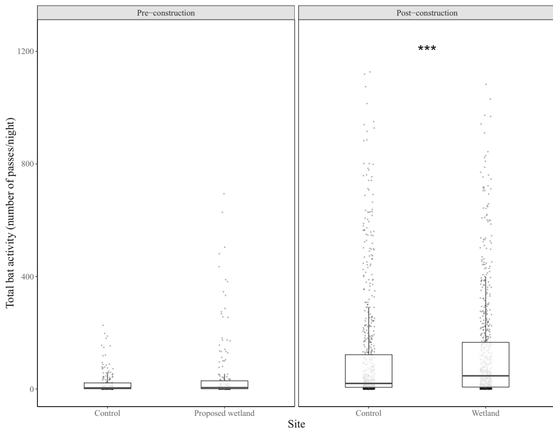
Fig. 1 Total bat activity (number of passes per night) in control and proposed wetland sites before the wetland construction (November 19th, 2016–March 14th, 2017) and in control and wetland sites after the construction (March 15th, 2017–March 28th, 2018) at the University of
