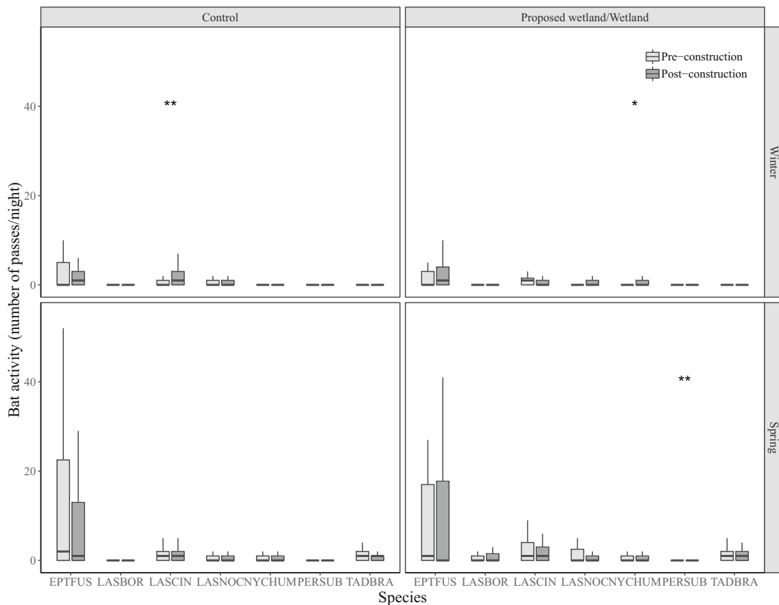
Fig. 4 Species specific bat activity (number of passes per night) in control and proposed wetland sites before the wetland construction in the Winter (November 19th, 2016–January 31st, 2017) and Spring (February 1st, 2017–March 14th, 2017), and in control and wetland sites after the construction in the Winter (November 19th, 2017–January 31st, 2018) and Spring (February 1st, 2018–March 14th, 2018) at the University of North Carolina Greensboro. Species abbreviations are: Eptesicus fuscus (EPTFUS), Lasiurus borealis (LASBOR), Lasiurus cinereus
