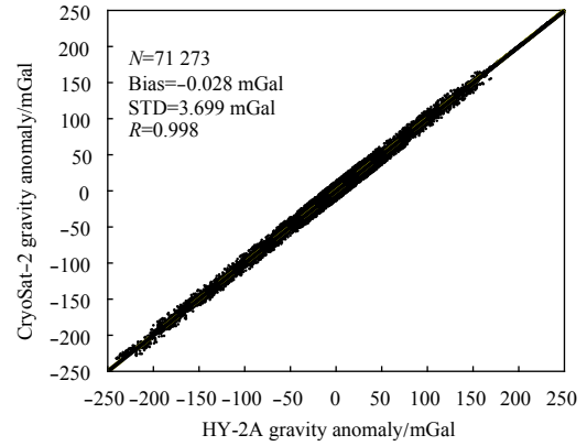
Fig. 2. Scatterplot of HY-2A gravity anomaly versus CryoSat-2 gravity anomaly near Taiwan Island.
