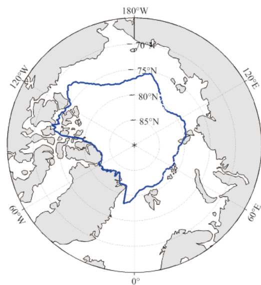
Fig. 4. Average of the minimum sea ice edge in 2002–2015.
