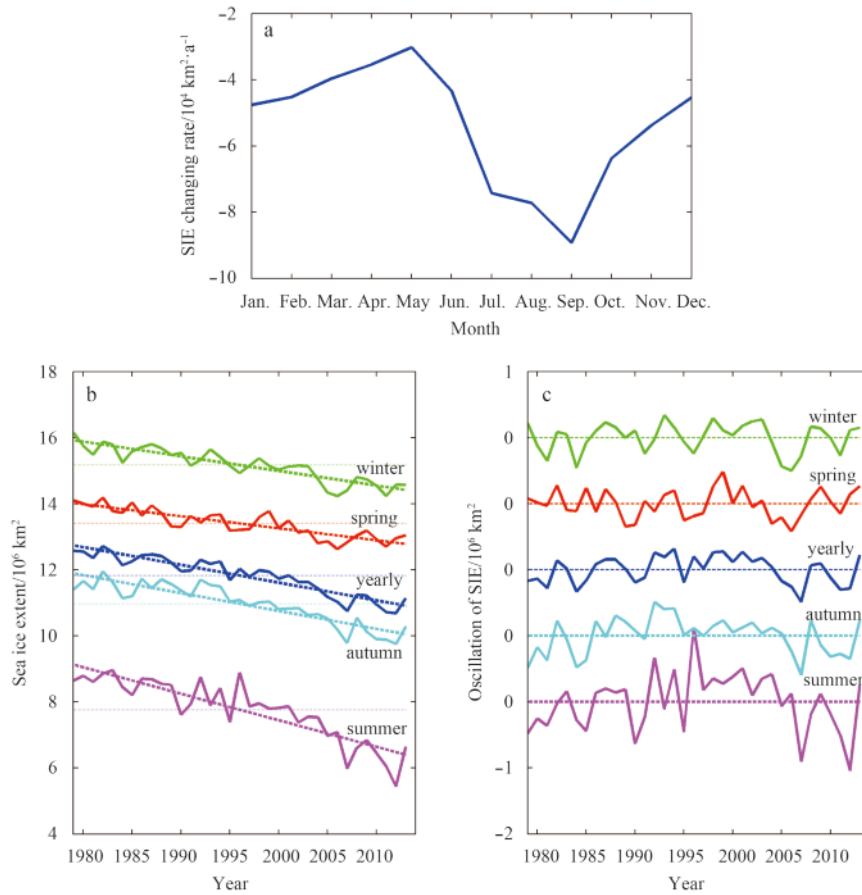
Fig. 2. Time series of sea ice extent from 1979 to 2013. a. Decline rate of linear trend for each month; b. average sea ice extents (solid curve) and their linear trends for all year round and for different seasons (dotted lines), and climatology sea ice extents in 1979–2013 (point line); and c. the long-term oscillation of sea ice extents with the linear trend removed for all year round and for each season.
