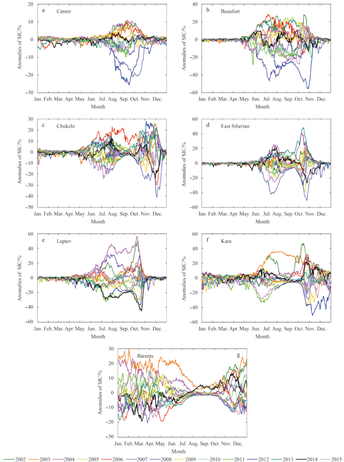
Fig. 7. Anomalies of the sea ice coverage for the central Arctic Ocean (a) and the marginal seas (b-g).
