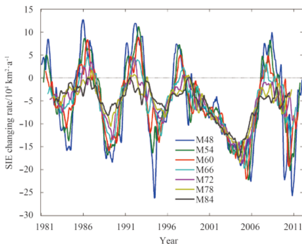
Fig. 3. Running linear trend using different windows width (e.g., M48 means a window width of 48 months) for sea ice extent anomaly.
