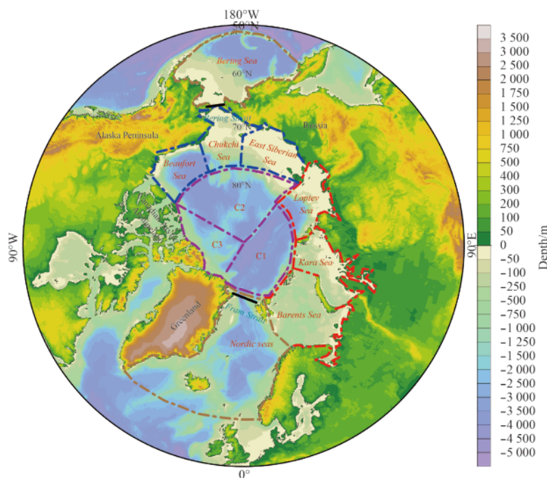
Fig. 1. Our definition of different regions in the Arctic Ocean.
