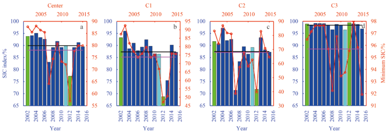
Fig. 9. The sea ice coverage indices during the melting-freezing period for the central Arctic Ocean and each adjacent sub-sea. The meaning of lines are same as Fig. 8.
