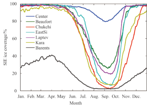
Fig. 6. The daily average for long-term variation of sea ice coverage for different divided regions.
