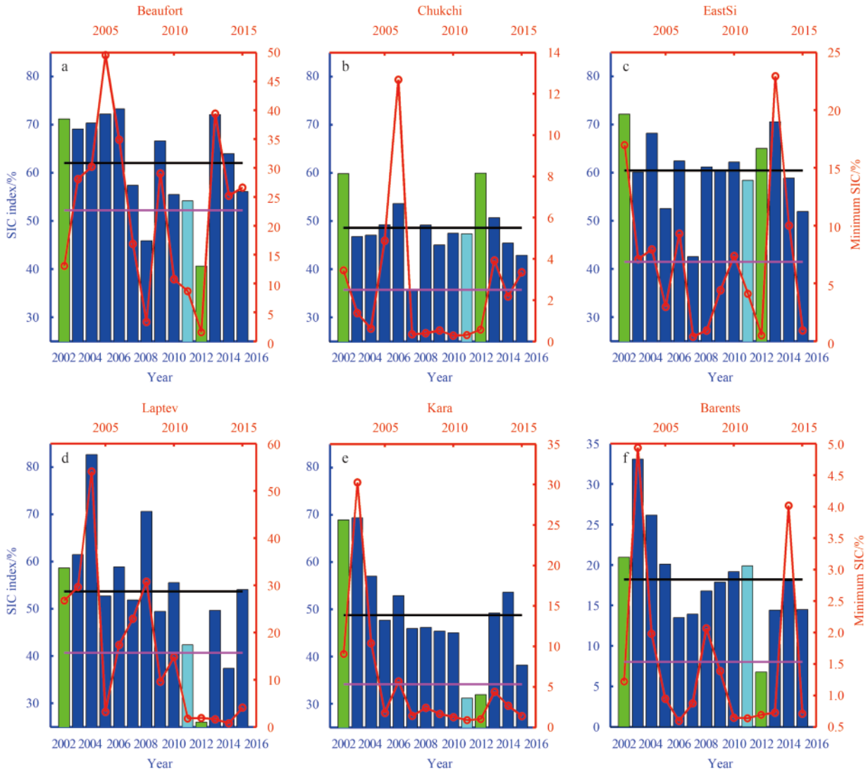
Fig. 8. The sea ice coverage indices during the melting-freezing period for each marginal sea. Due to data breach for almost one year, the indices of sea ice coverage in the freezing period (the green bar) and melting period (the light blue bar) may be incomplete. Although the indices may include the changes of the maximum and minimum sea ice extent, the mean value may have a large deviation. The red dot-line represents the minimum sea ice coverage for each year, the black line the long-term mean of sea ice coverage, and the purple line the long-term mean of minimum sea ice coverage. Notice that the sea ice coverage of the Barents Sea has a different magnitude to the other marginal sea.
