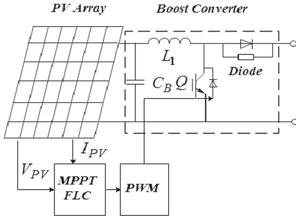
Fig. 3 Boost circuit and MPPT for the PV
