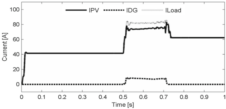
Fig. 23 Current of the PV (solid), DG (dotted) and the current required (dashed)
