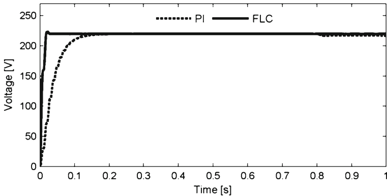
Fig. 19 Voltage RMS at the PCC
