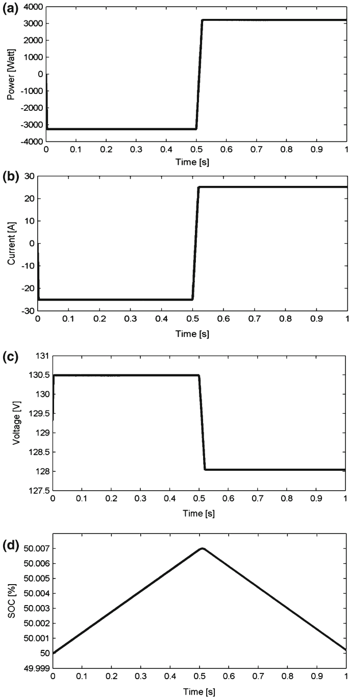
Fig. 15 Battery response a power, b current, c voltage, d SOC
