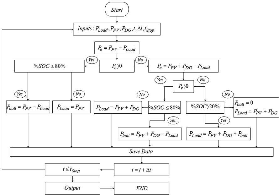
Fig. 12 Flowchart of the SCS
