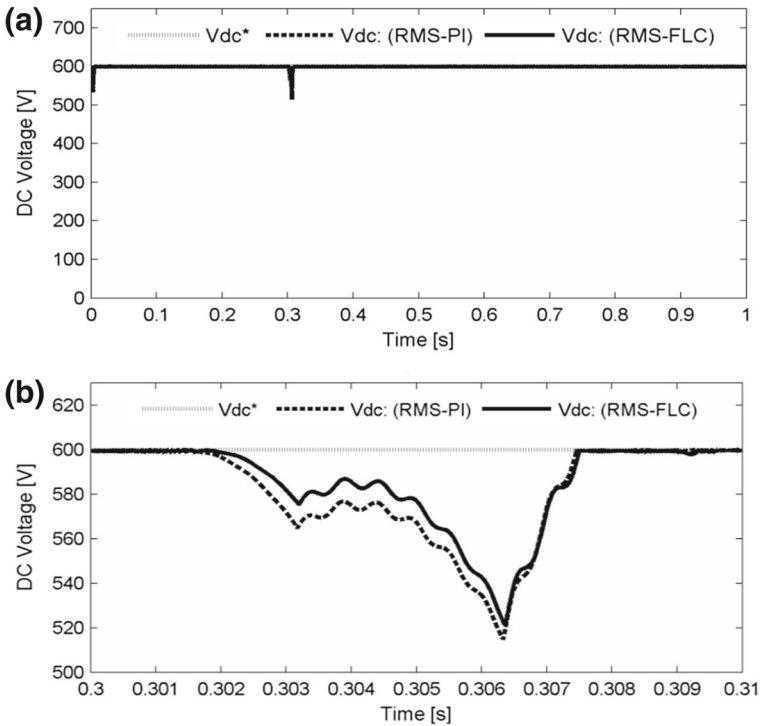
Fig. 30 a DC voltage with FLC (solid), PI (dotted), reference (dashed) and b Zoom of (a)
