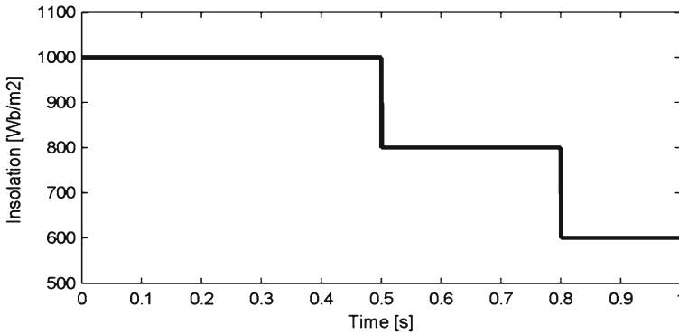
Fig. 13 Simulated changes in the solar irradiance
