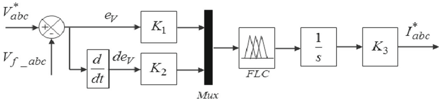
Fig. 10 FLC structure of voltage controller
