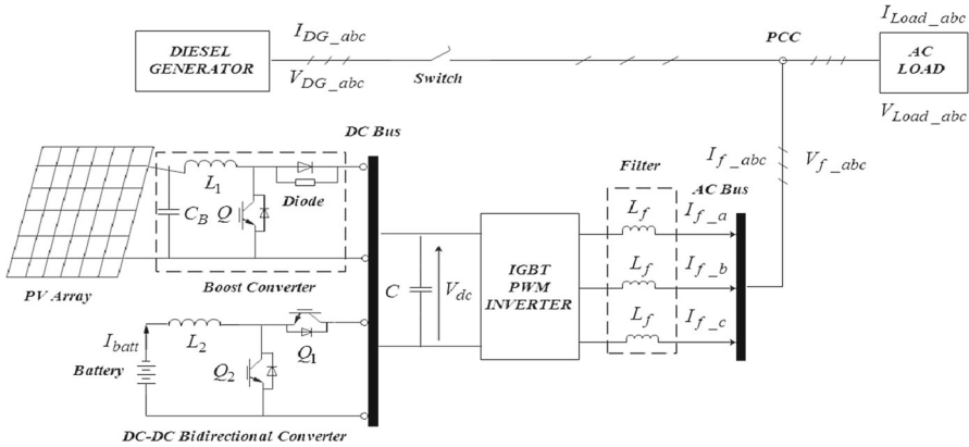
Fig. 1 Proposed standalone HPS
