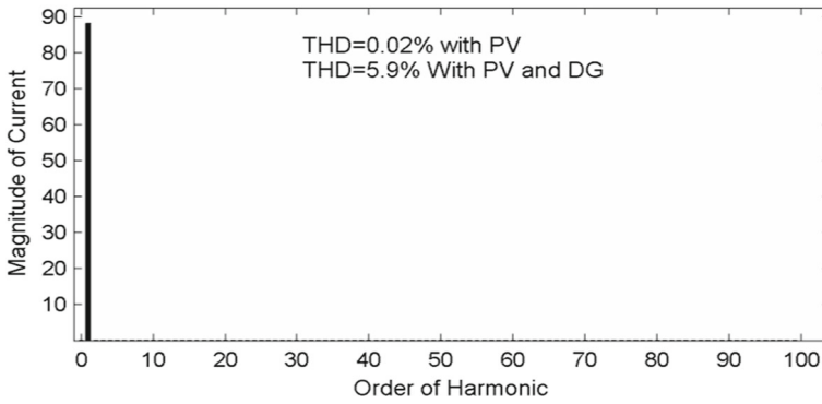
Fig. 25 THD of the current
