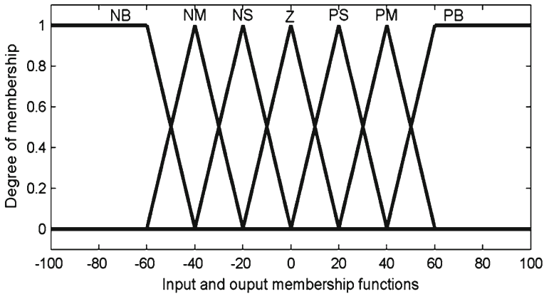
Fig. 11 MFs of the FLC voltage controller
