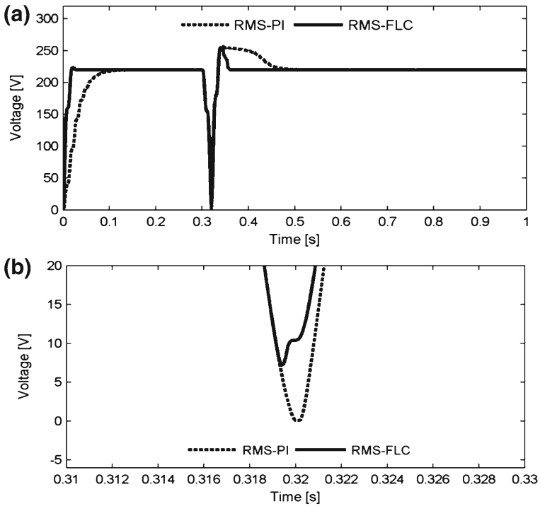
Fig. 29 a RMS of the voltage at PCC and b zoom of (a)
