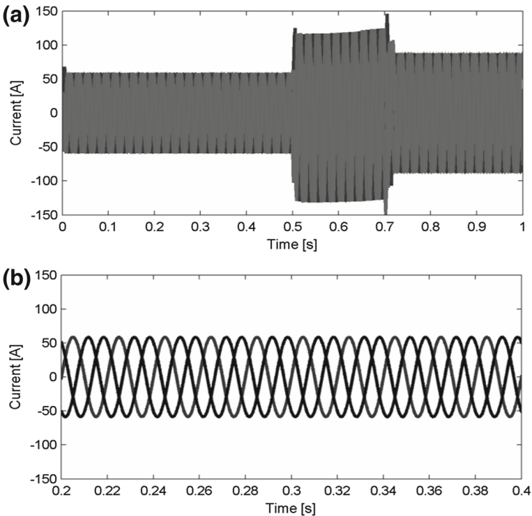
Fig. 24 a Load current waveforms and b zoom of (a)
