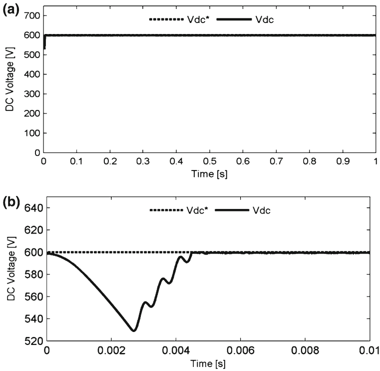
Fig. 16 a DC voltage and b zoom of (a)
