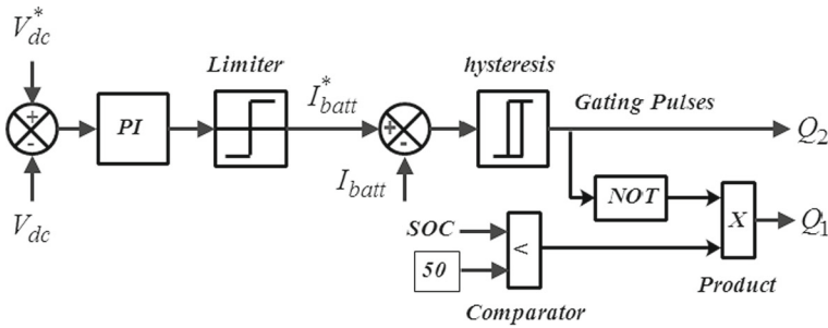
Fig. 7 Overall arrangement of the battery converter controller
