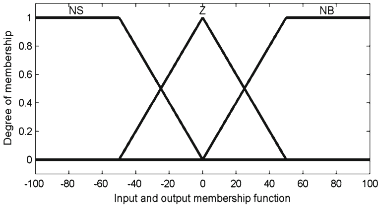
Fig. 5 MFs of the MPPT_FLC
