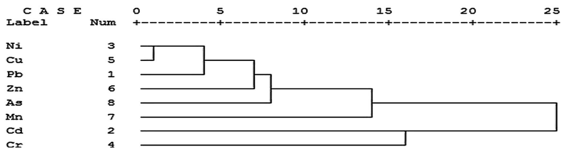
Fig. 2 Hierarchical clustering results (dendrogram) of the heavy metal concentrations in sediment and water samples of Dhalai Beel and Bangshi River
