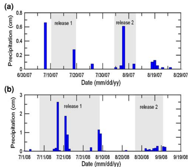
Fig. 7 Time-series plots of daily precipitation during a 2007 and b 2008 field seasons. Gray areas indicate timing of CO 2 releases
