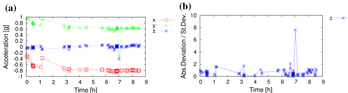
Fig. 8 a VD estimations against time with a wrong estimation performed while driving, b absolute deviation over standard deviation ratio on the z axis
