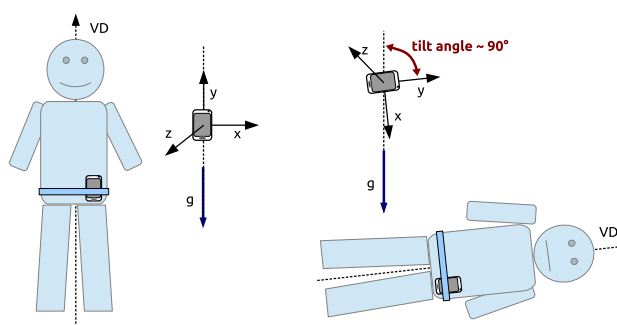
Fig. 1 Lying posture detection with aligned device. In this example, VD is aligned with the y axis of the device. The tilt angle between y and gravity is measured and compared against a threshold (e.g. 50°) in order to detect postural transitions from standing to lying
