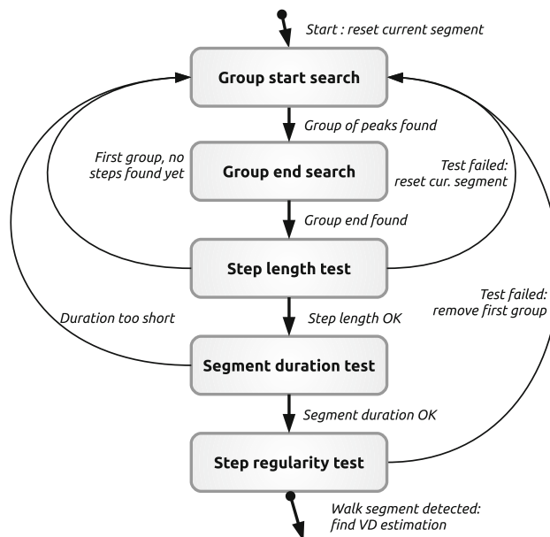
Fig. 5 Walk detection as a finite state machine
