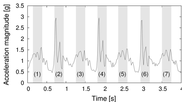
Fig. 4 Example of acceleration pattern during a short walk: the groups of peaks produced by each step have been highlighted and numbered
