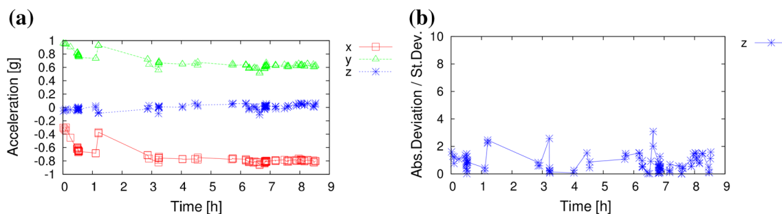
Fig. 7 a VD estimations against time, b absolute deviation over standard deviation ratio on the z axis
