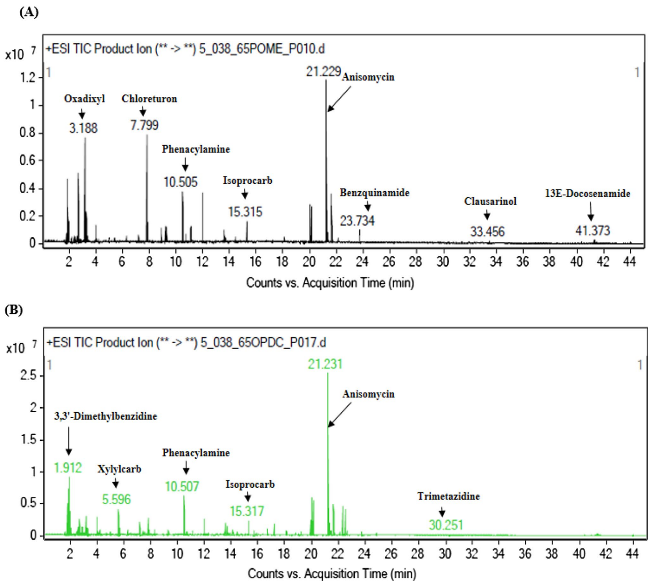
Fig. 4 Mass spectra showing antimicrobial agents emitted by S. philanthi RM-1-138 produced A in palm oil mill effluent (POME) and B on oil palm decanter cake (OPDC) medium detected by LC-Q-TOF MS/MS analysis
