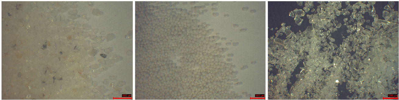
Fig. 1 Silica sand ( left ), glass spheres ( centre ) and glass particles ( right ) under stereoscope ( \times 8 for all cases)
