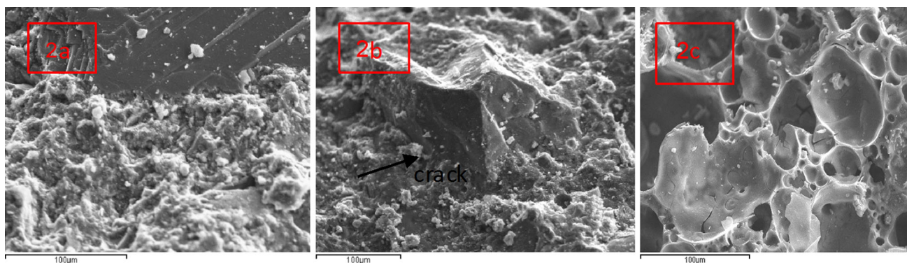
Fig. 2 SEM images of A sample with strong sand-cement interface (a), crack in the circumference of a glass grain and the matrix in B sample (b) and porous structure in C sample (c)
