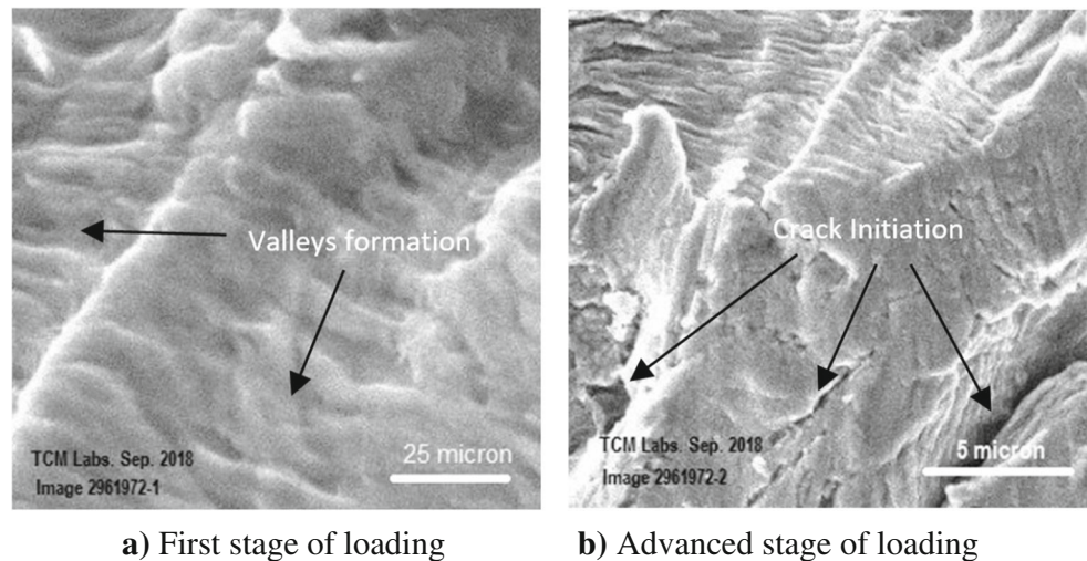
Fig. 5 Micro observation of the gained crack initiation
