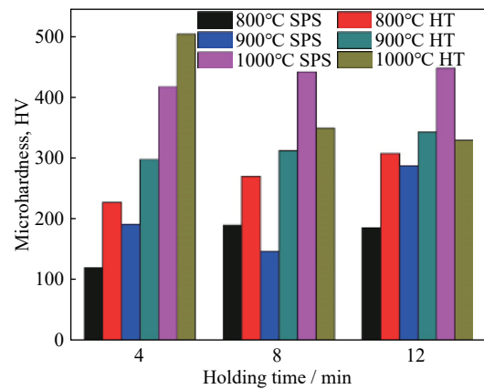
Fig. 6. Comparative microhardness graph of SPS and heat-treated (HT) sintered \text{Al}_{20}\text{Cr}_{20}\text{Fe}_{25}\text{Ni}_{25}\text{Mn}_{10} alloys.
